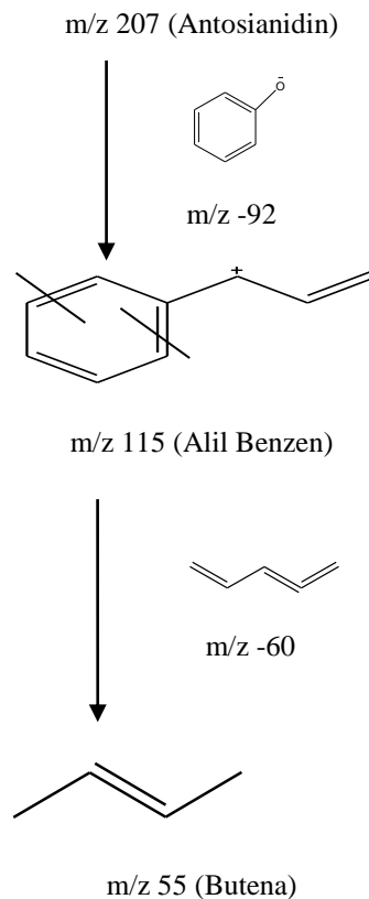
Gambar 4.5 Fragmentasi Antosianidin
