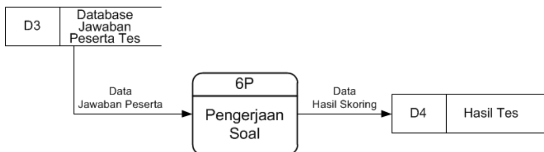
Gambar 4. 22. DFD Level 1 Proses 6
