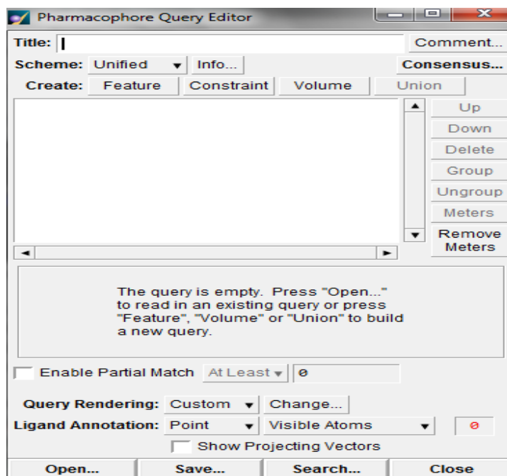
Gambar III.4 Tampilan panel Pharmacophore Query Editor
