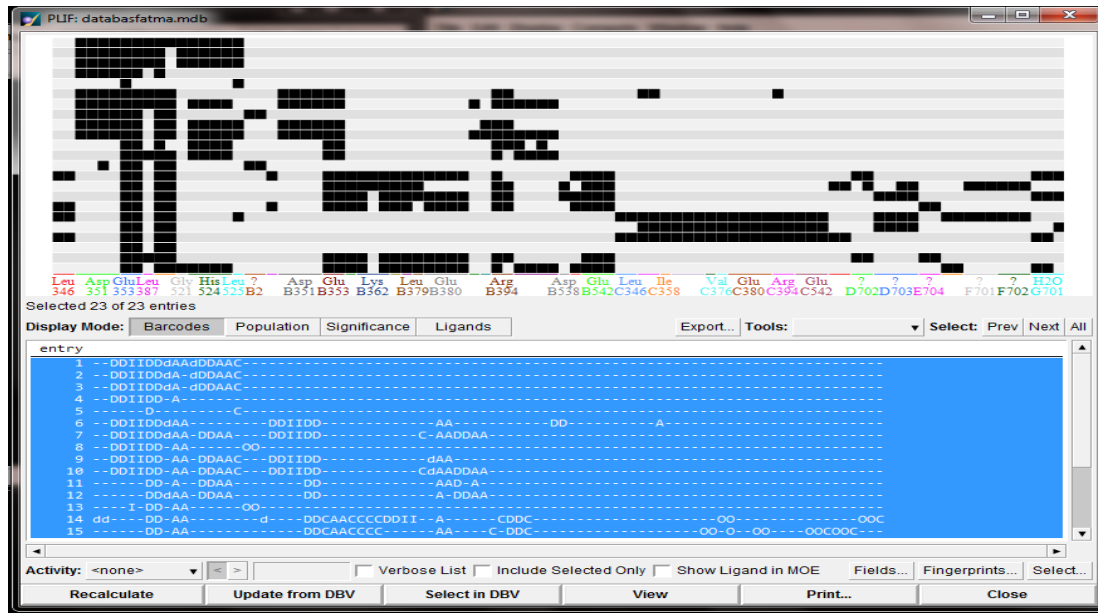
Gambar III.3 Panel PLIF 23 Protein ER- \alpha
