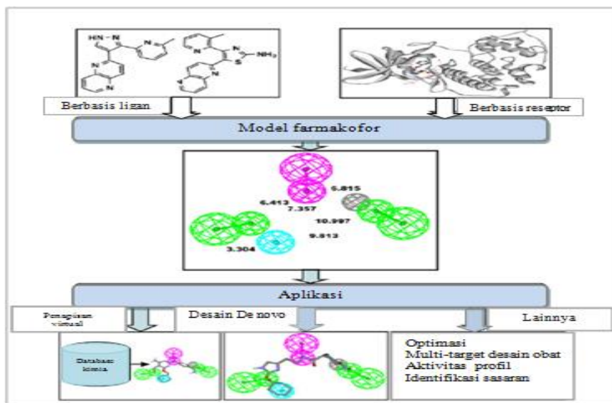
Gambar II.3 Struktur Model Farmakofor
