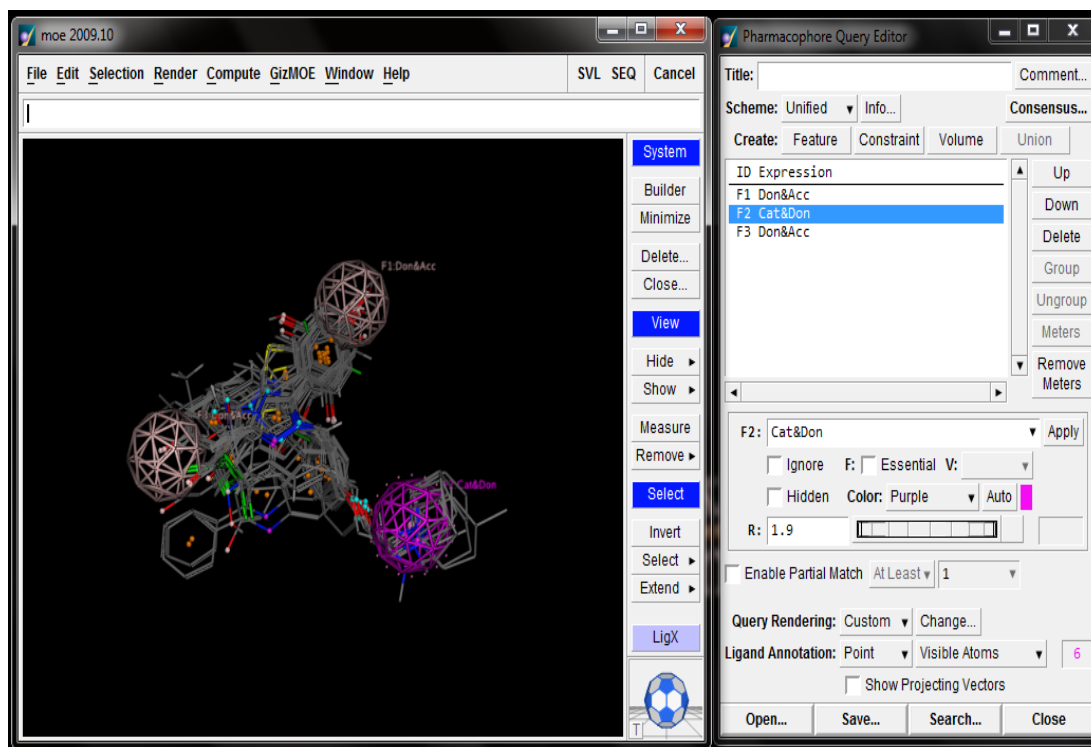
Gambar III.5 Tampilan fitur-fitur farmakofor senyawa 23 dan panel Pharmacophore Query Editor
