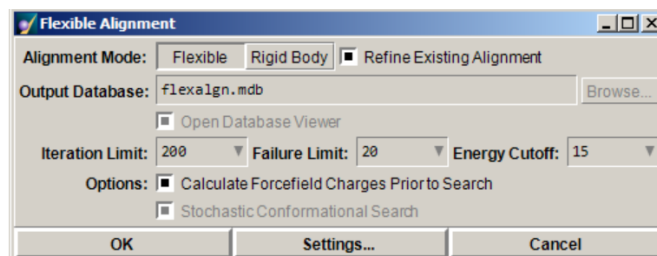
Gambar III.6 Panel Flexible Alignment
