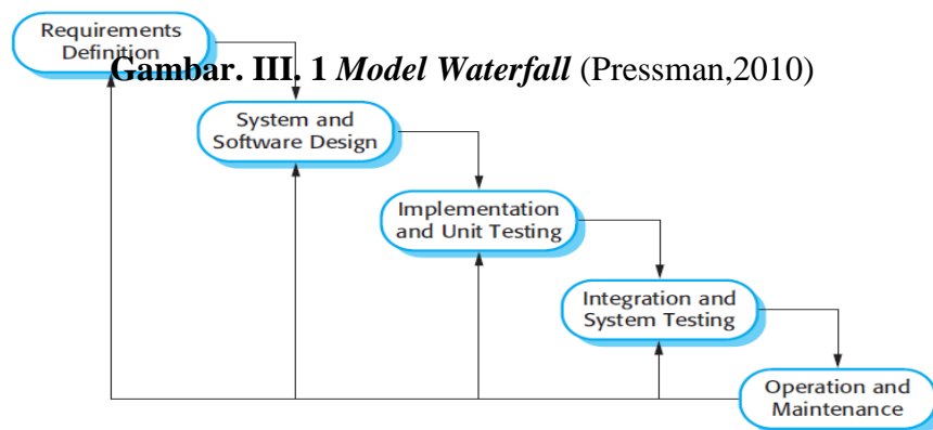
Gambar III. 1 Model Waterfall
