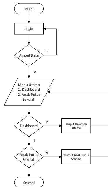
Gambar IV.20 Flowchart Petugas
