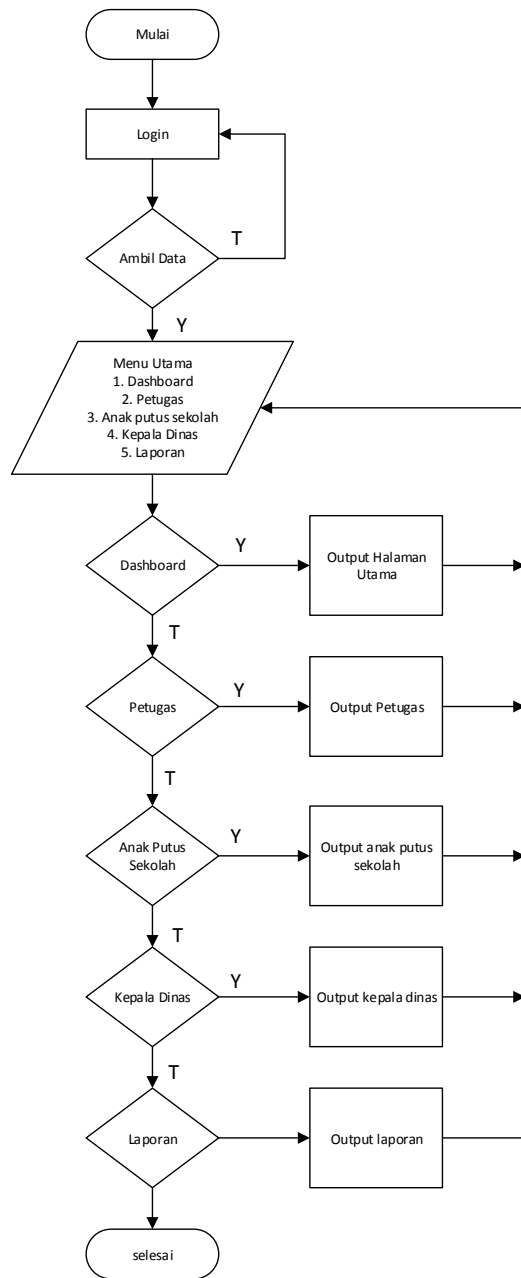
Gambar IV. 20 Flowchart Admin
