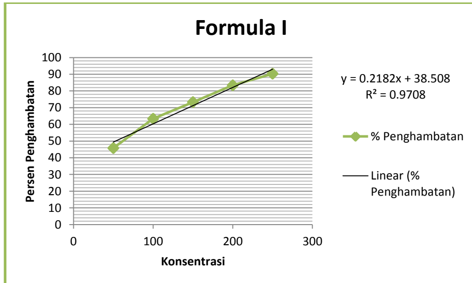
Gambar 13. Sirup Formula I terhadap DPPH
