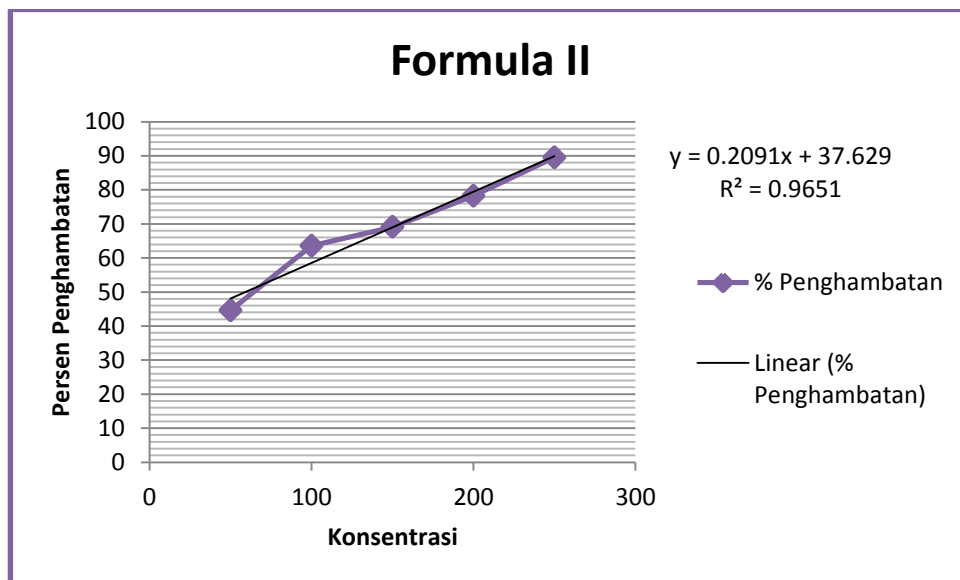
Gambar 14. Sirup Formula II terhadap DPPH
