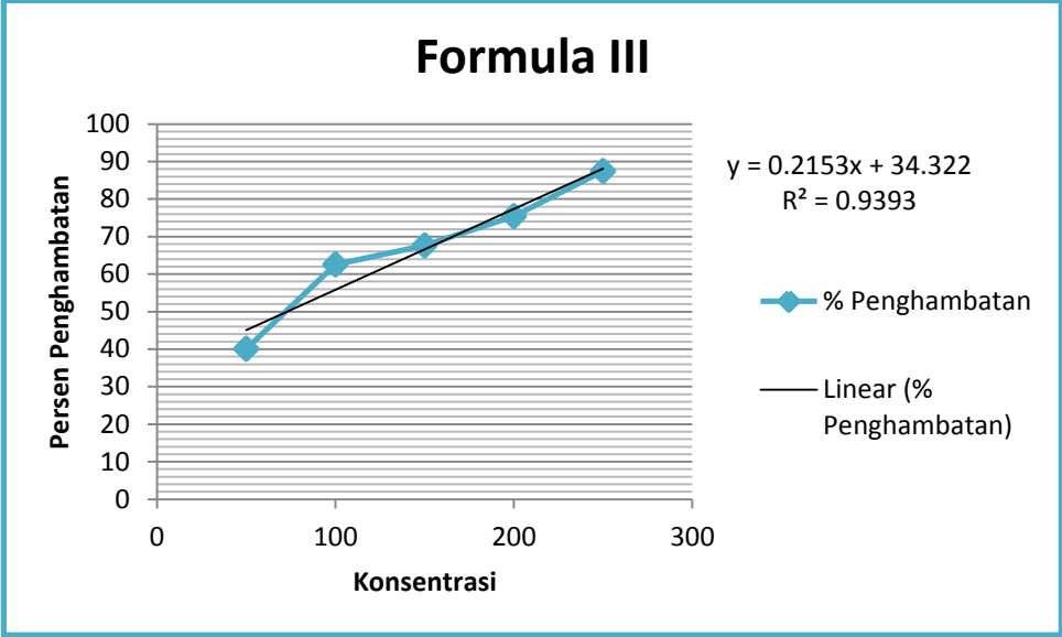
Gambar 15. Sirup Formula III terhadap DPPH
