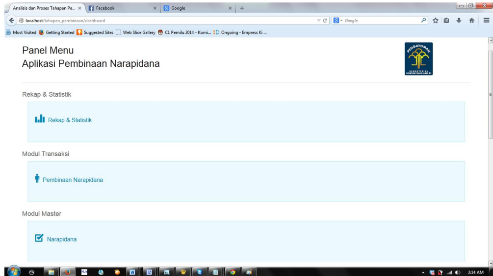
Gambar V.3. Menu Dashboard
