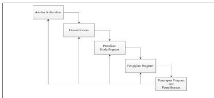
Gambar III.1. Model Waterfall
