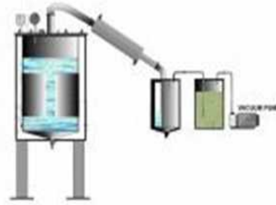
Gambar II.11 Rangkaian Alat Distilasi Vakum
