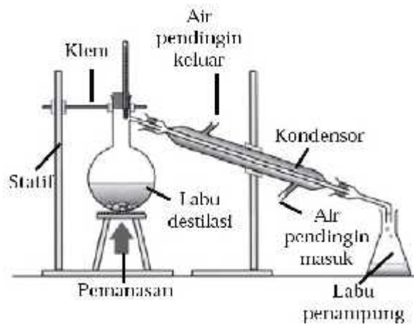
Gambar II.10 Rangkaian Alat Distilasi Uap
