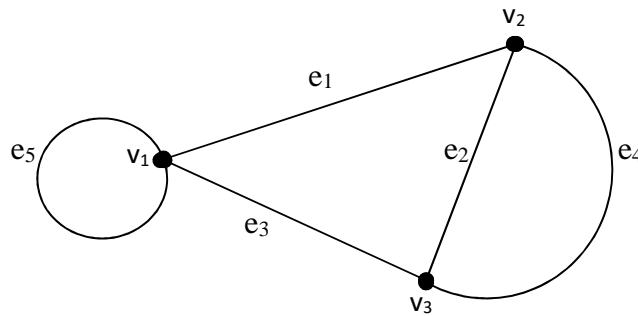
Gambar 2.2 pseudograf
