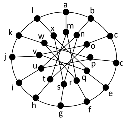
Gambar 4.6 Graf Nauru ( G_2 )
