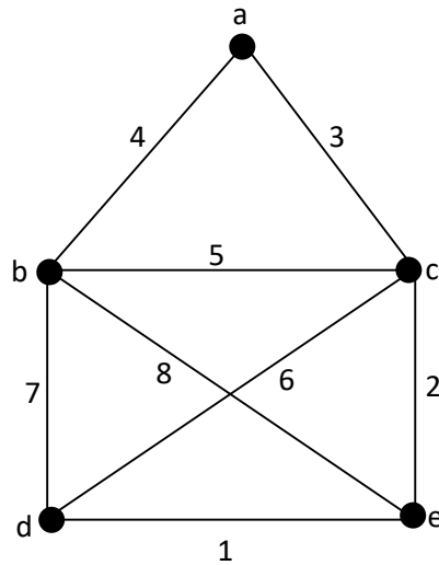
Gambar 2.21 lintasan Eulerian. 11
