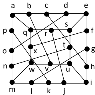
Gambar 4.3 Graf Nauru ( G_3 )
