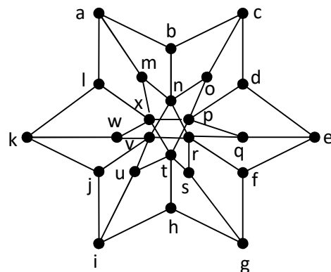
Gambar 4.4 Graf Nauru ( G_4 )
