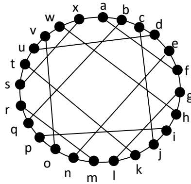
Gambar 4.5 Graf Nauru ( G_1 )
