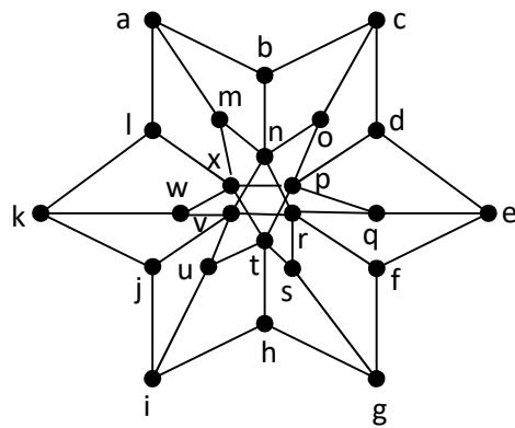
Gambar 4.8 Graf Nauru ( G_4 )
