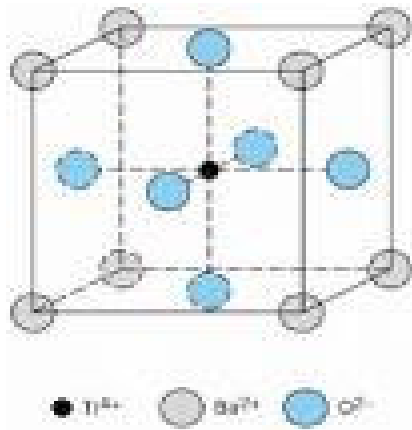
Gambar 9. simple cubic
