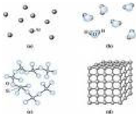
Gambar 10. Body-centered cubic 23
