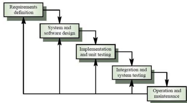
Gambar III 1 Model Waterfall (Pressman, 2001)
