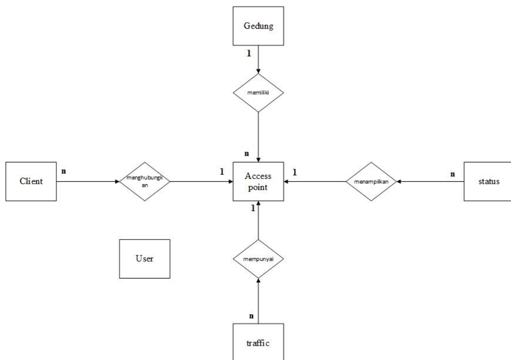
Gambar IV.6 Entity Relational Diagram (ERD)
