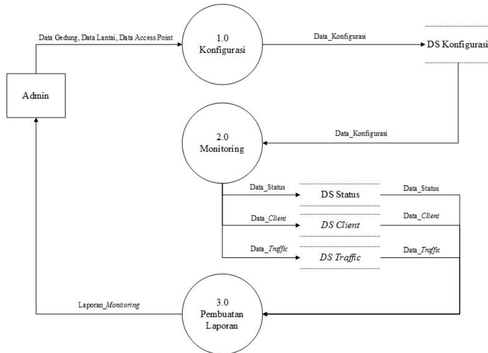
Gambar IV.5 DFD Level 1
