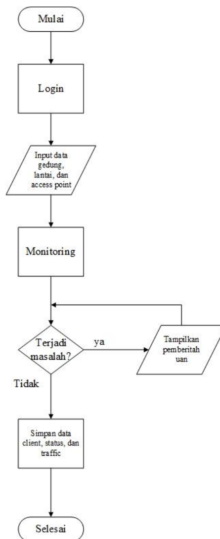
Gambar IV.9 Flowchart Diagram
