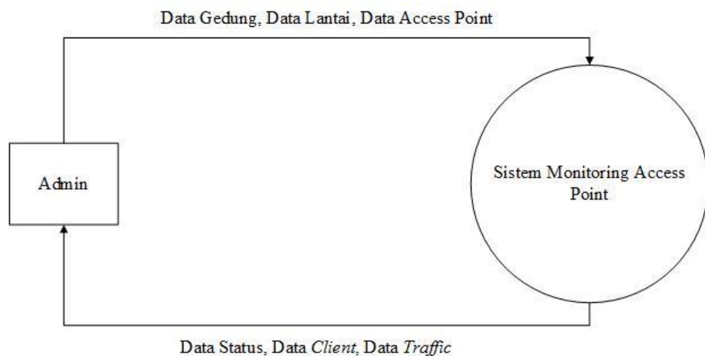
Gambar IV.3 Context Diagram
