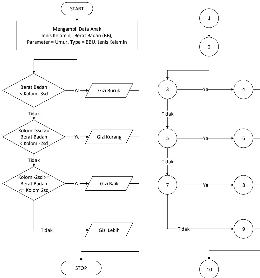
Gambar V. 10 Pengujian Penilaian Status Gizi
