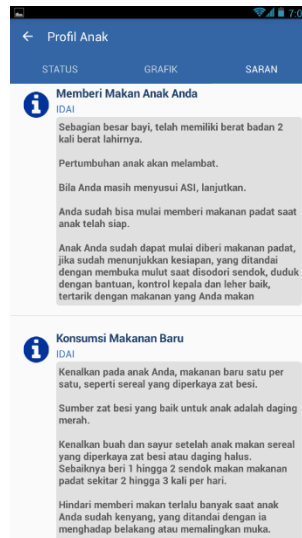
Gambar V. 4 Antarmuka Saran
