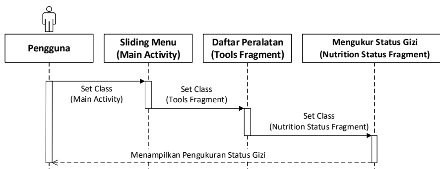
Gambar IV. 8 Sequence Diagram Mengukur Status Gizi
