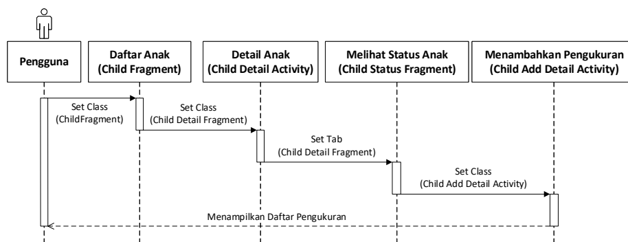
Gambar IV. 4 Sequence Diagram Menambah Pengukuran
