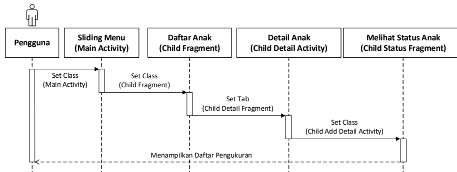
Gambar IV. 3 Sequence Diagram Membuka Detail Anak
