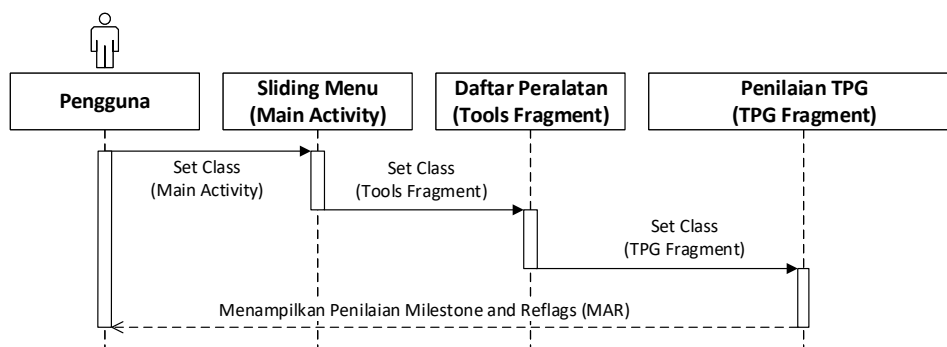
Gambar IV. 11 Sequence Diagram Mengukur TPG
