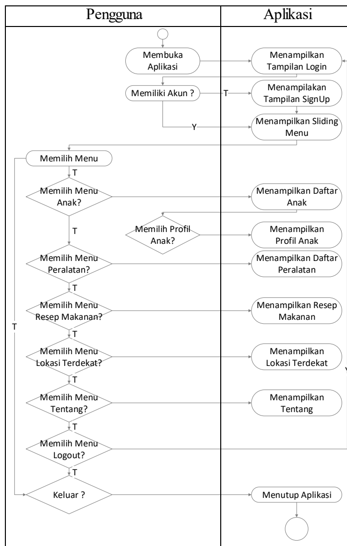
Gambar IV. 15 Activity Diagram Sliding Menu
