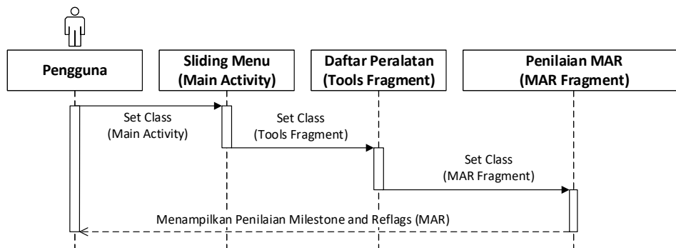
Gambar IV. 10 Sequence Diagram Menilai Redstone and Redflags (MAR)
