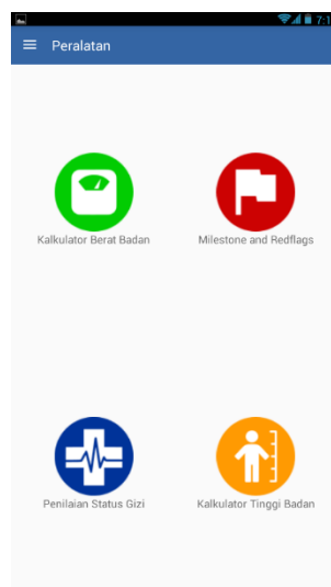
Gambar V. 5 Antarmuka Tools
