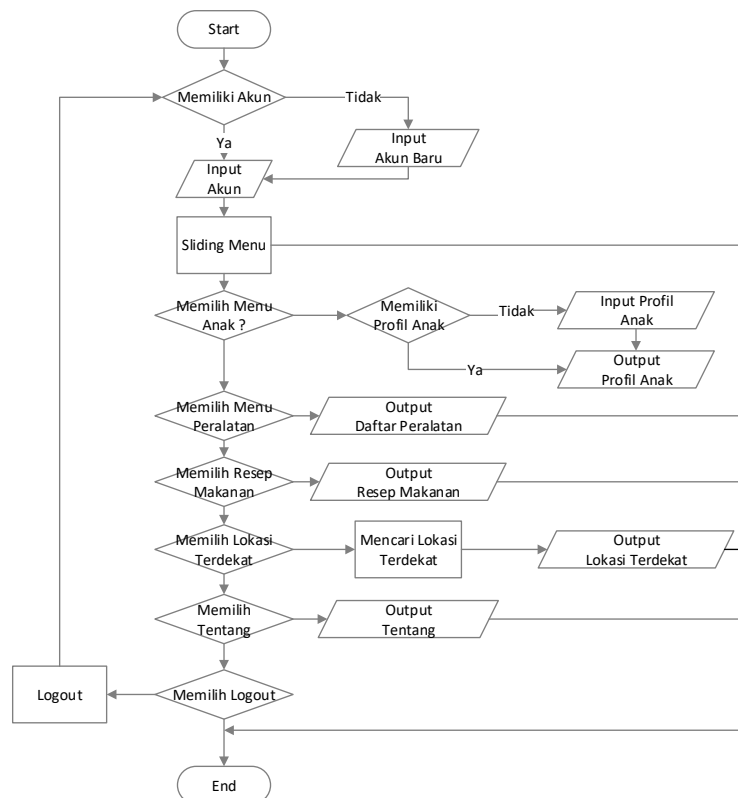
Gambar IV. 16 Flowchart (Alur Program)
