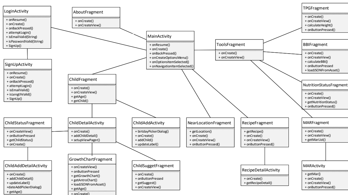
Gambar IV. 2 Class Diagram
