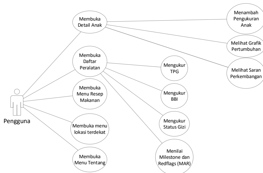
Gambar IV. 1 Use Case Diagram
