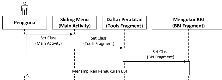
Gambar IV. 9 Sequence Diagram Mengukur BBI
