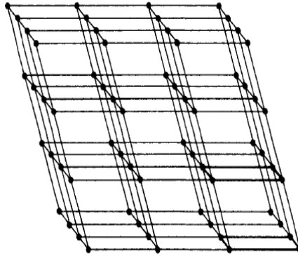
Gambar 6. Point lattice
