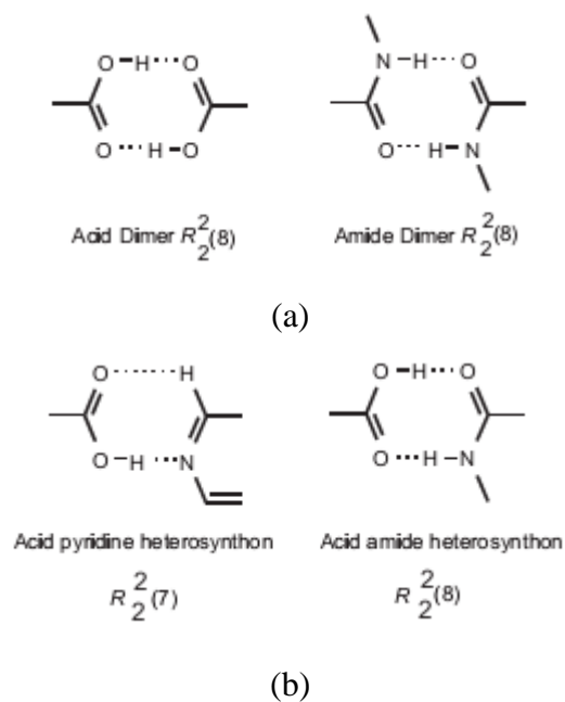
Gambar 9. Synthon supramolekular (a) homosynthon , (b) heterosynthon
