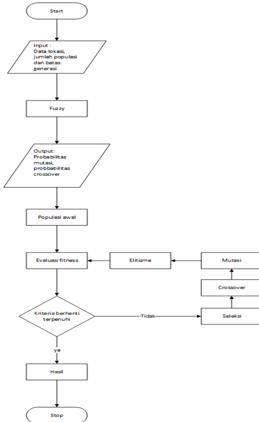
Gambar IV. 5 Flowchart
