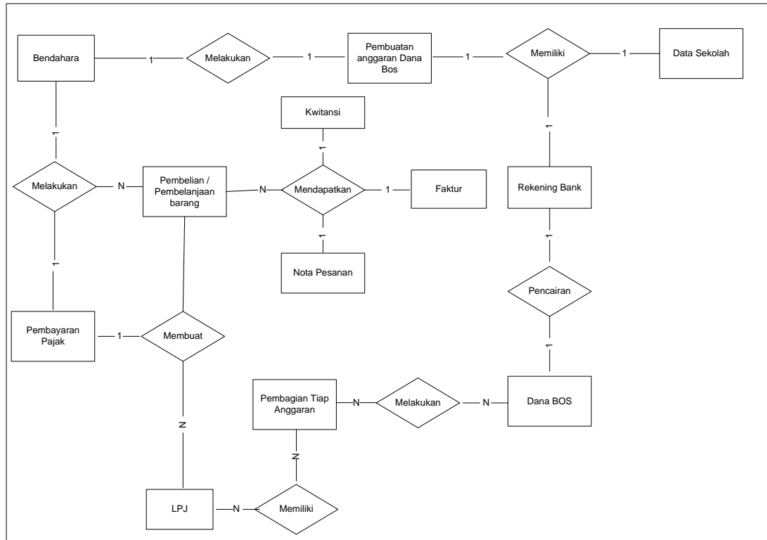
Gambar IV. 8 Diagram ERD
