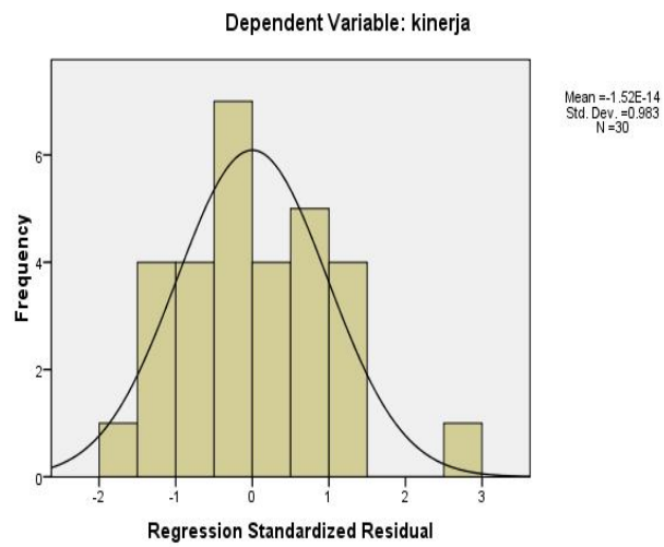
Histogram
