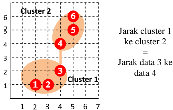
Gambar 1.3 Ilustrasi Single Linkage
