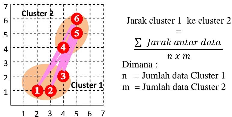
Gambar 1.5 Ilustrasi Average Linkage
