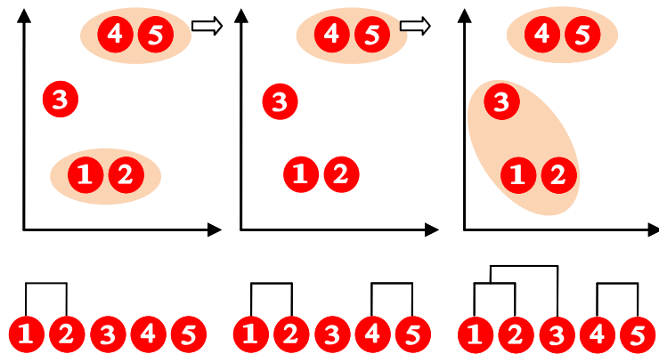
Gambar 1.2 Ilustrasi Algoritma Hierarchical Clustering
