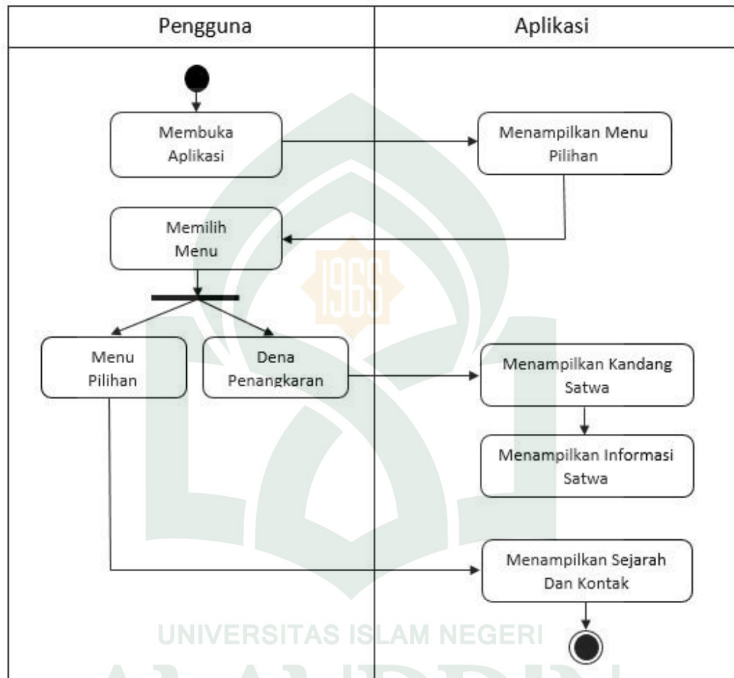
Gambar IV.11. Activity Diagram aplikasi penangkaran satwa Bontomarannu Education Park
