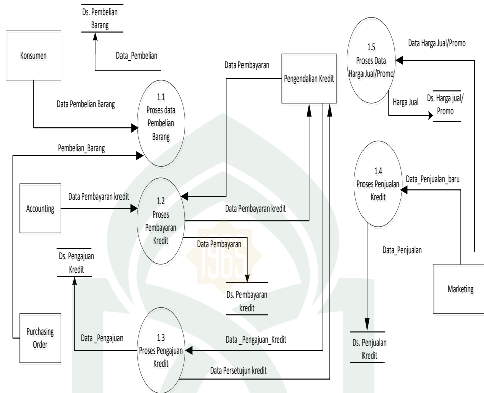
Gambar IV.6 Data Flow Diagram Level II Proses 1
