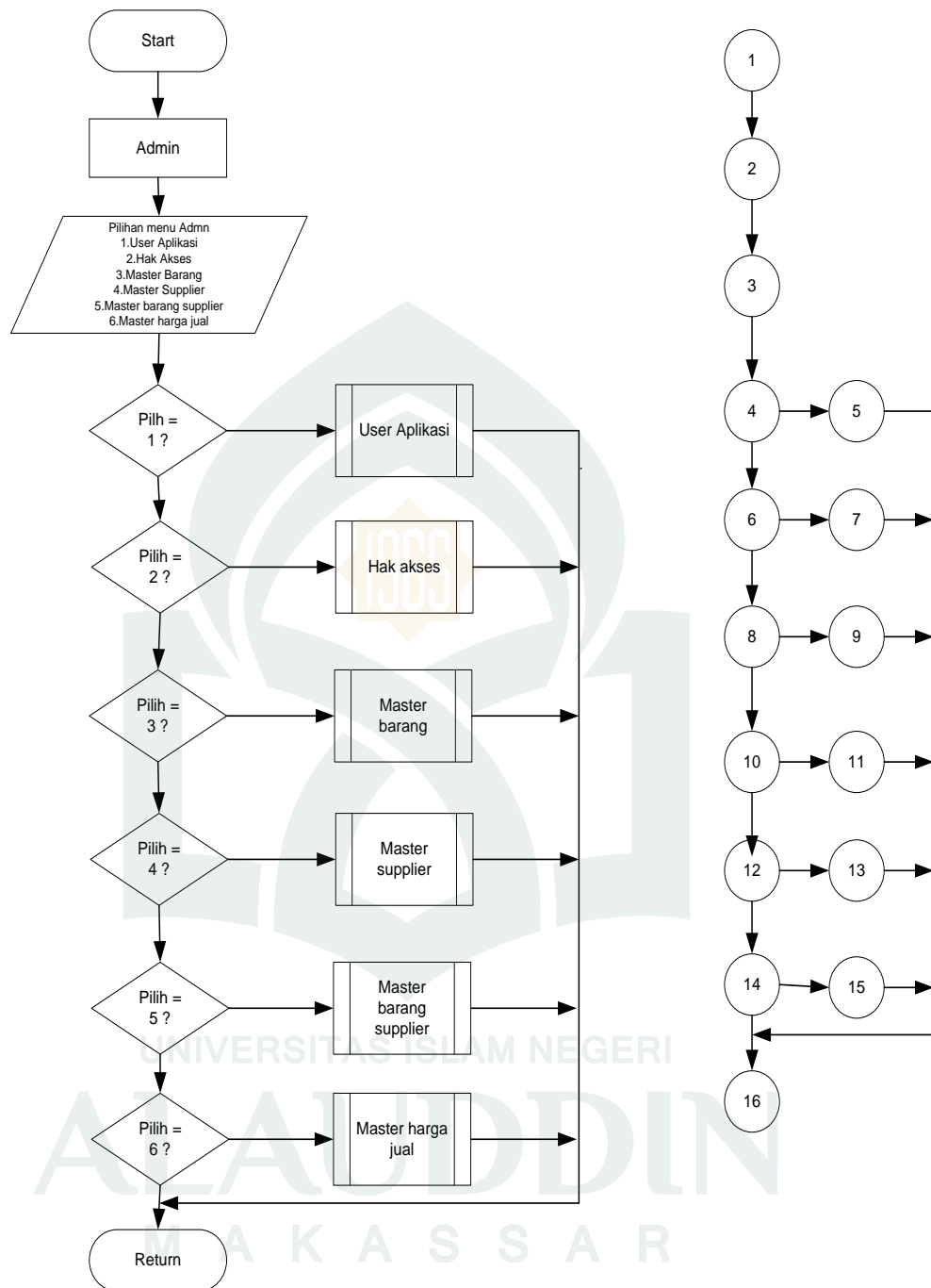
Gambar V.14 Flowchart dan Flowgraph Menu Admin
