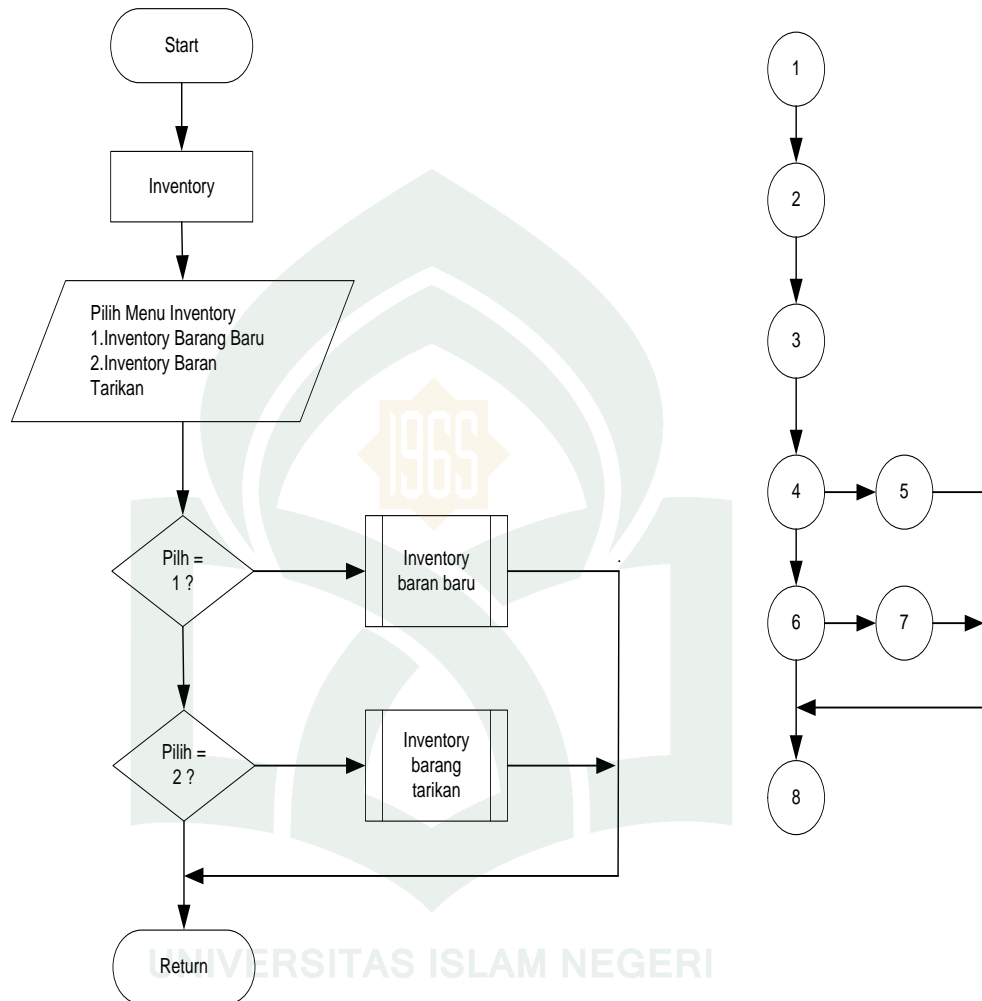
Gambar V.11 Flowchart dan Flowgraph Menu Inventory
