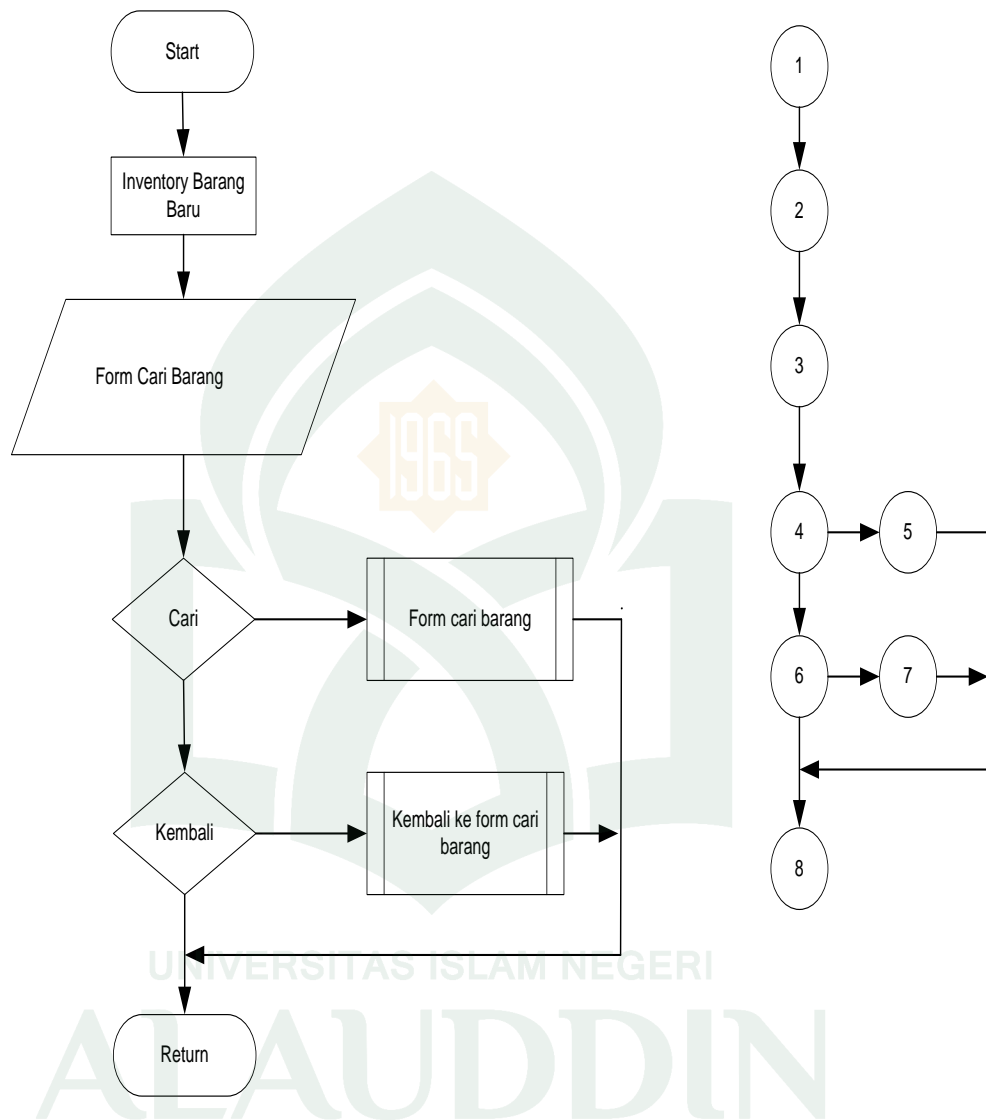
Gambar V.12 Flowchart dan Flowgraph Sub Menu Inventory Barang
