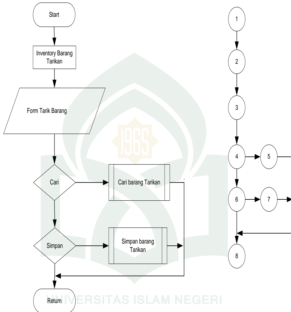
Gambar V.16 Flowchart dan Flowgraph Sub Menu Inventory Barang
