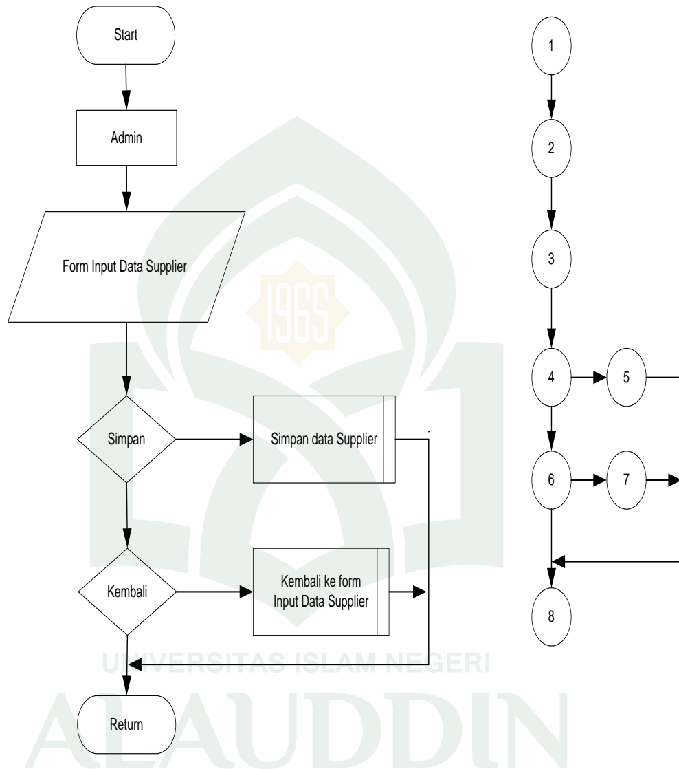
Gambar V.23 Flowchart dan Flowgraph Sub Menu Master Supplier
