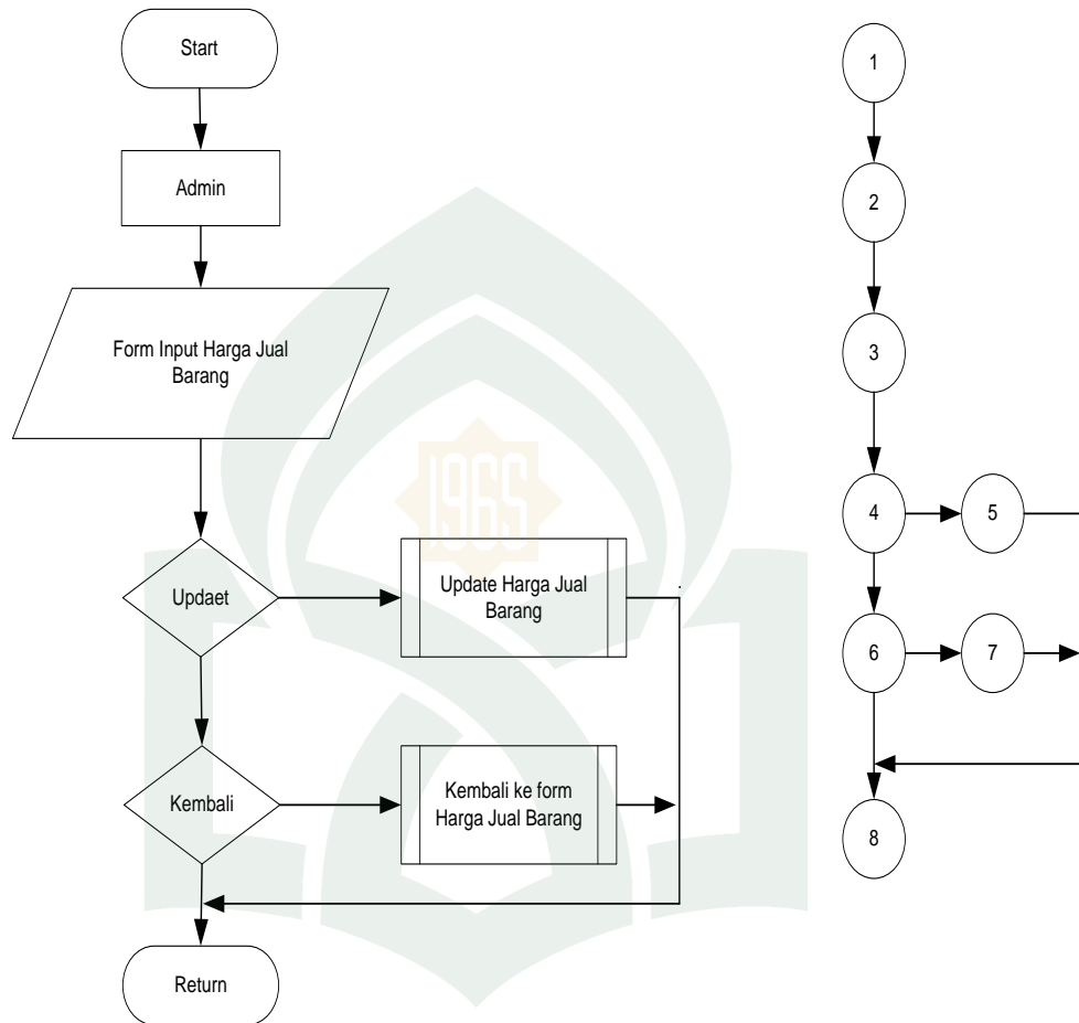
Gambar V.27 Flowchart dan Flowgraph Sub Menu Master Harga Jual
