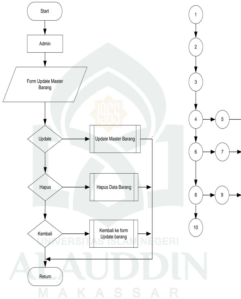
Gambar V.22 Flowchart dan Flowgraph Sub Menu Master Barang Form
