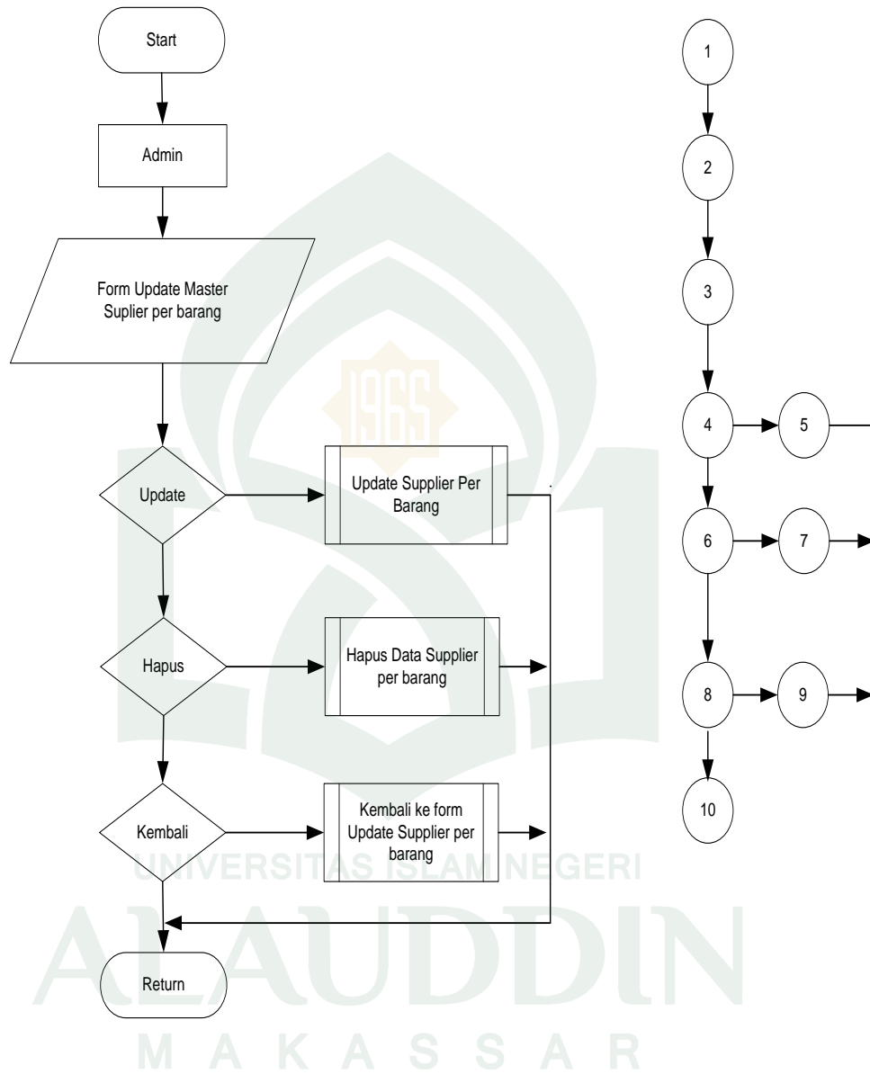
Gambar V.26 Flowchart dan Flowgraph Sub Menu Master Barang
