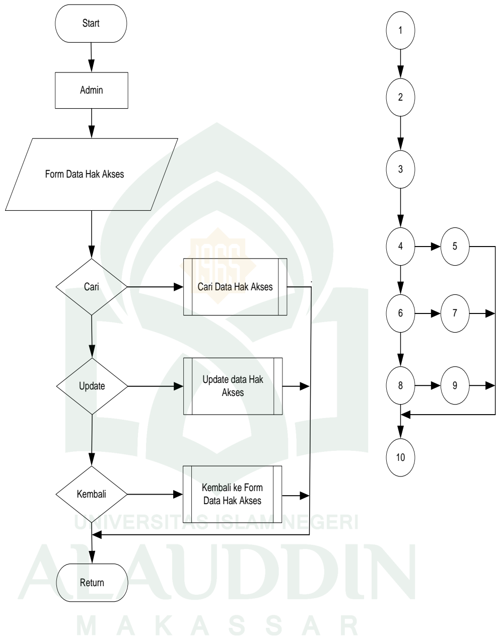
Gambar V.20 Flowchart dan Flowgraph Sub Menu Hak Akses
