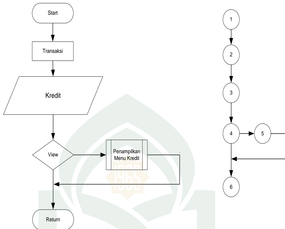
Gambar V.6 Flowchart dan Flowgraph Sub Menu Kredit
