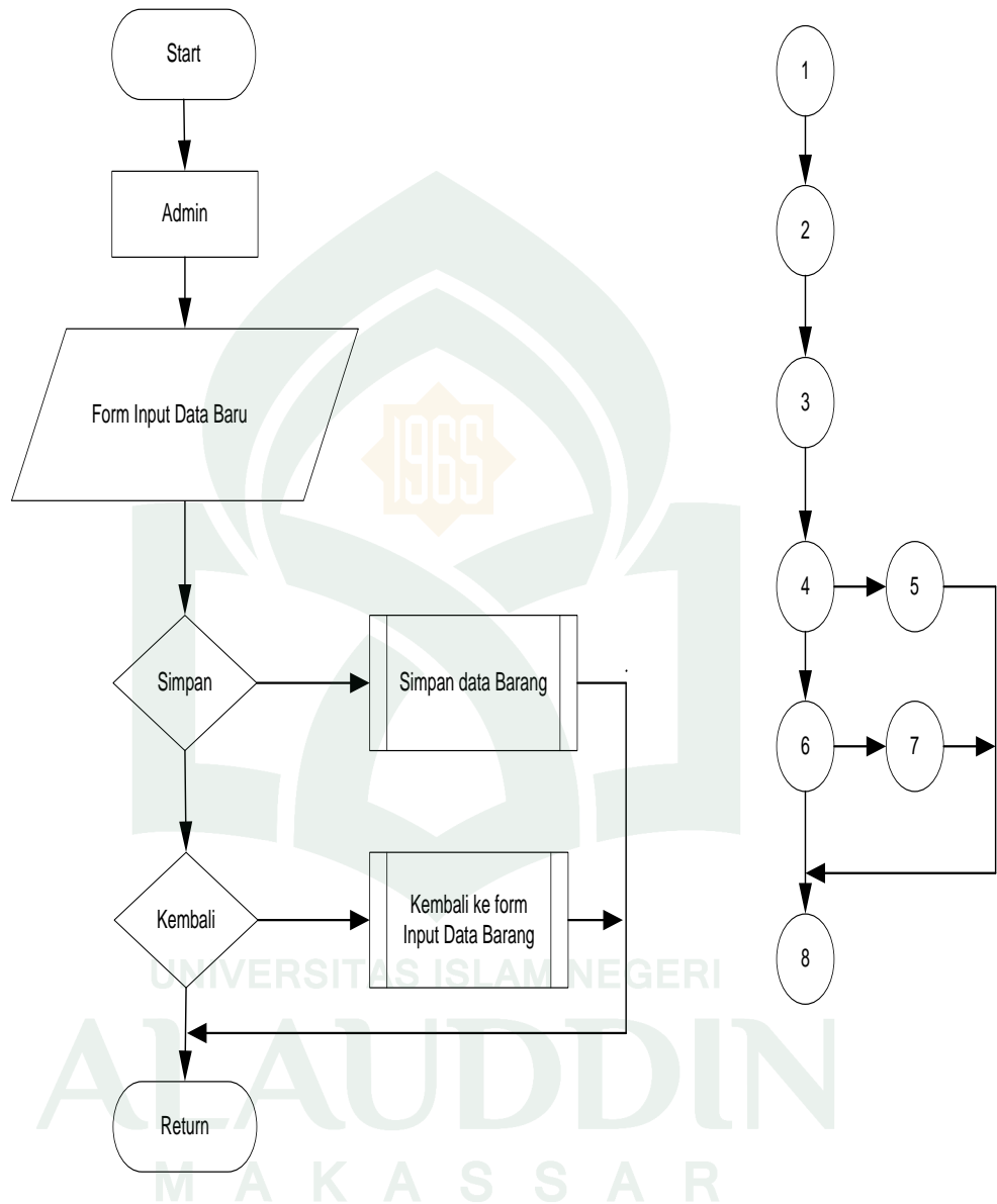
Gambar V.21 Flowchart dan Flowgraph Sub Menu Master Barang Form
