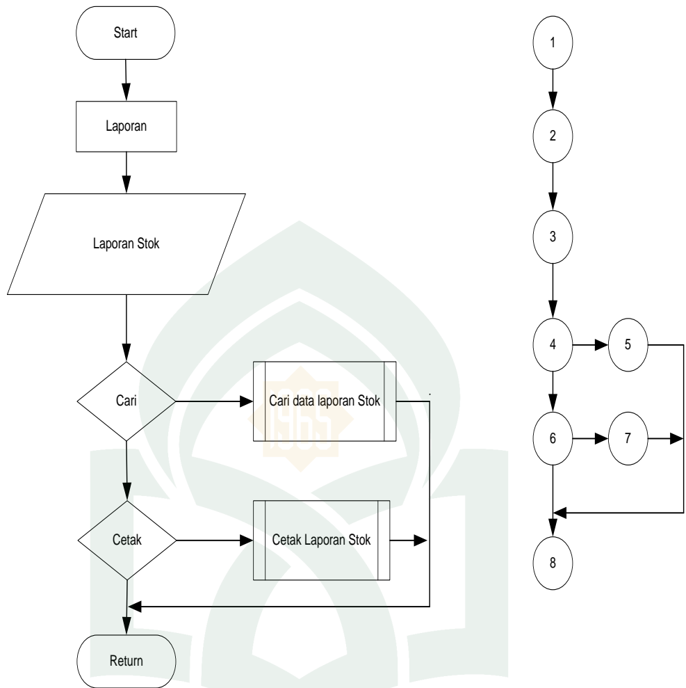
Gambar V.30 Flowchart dan Flowgraph Sub Menu Laporan Stok
