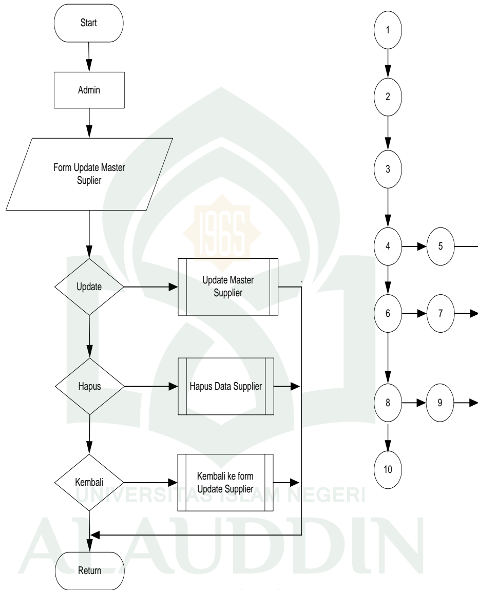
Gambar V.24 Flowchart dan Flowgraph Sub Menu Master Supplier
