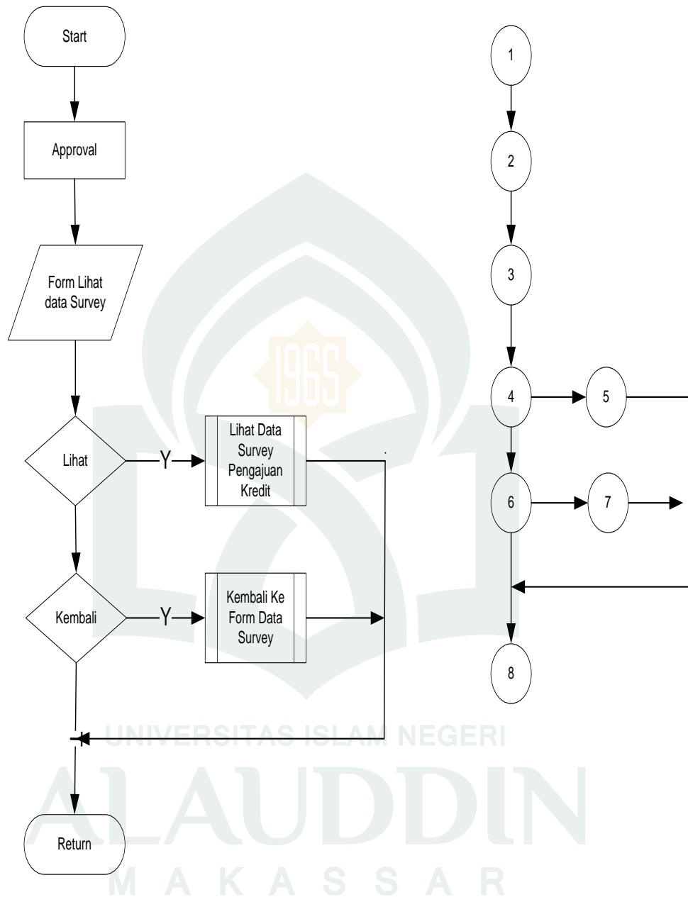
Gambar V.10 Flowchart dan Flowgraph Sub Menu Approval Form Lihat
