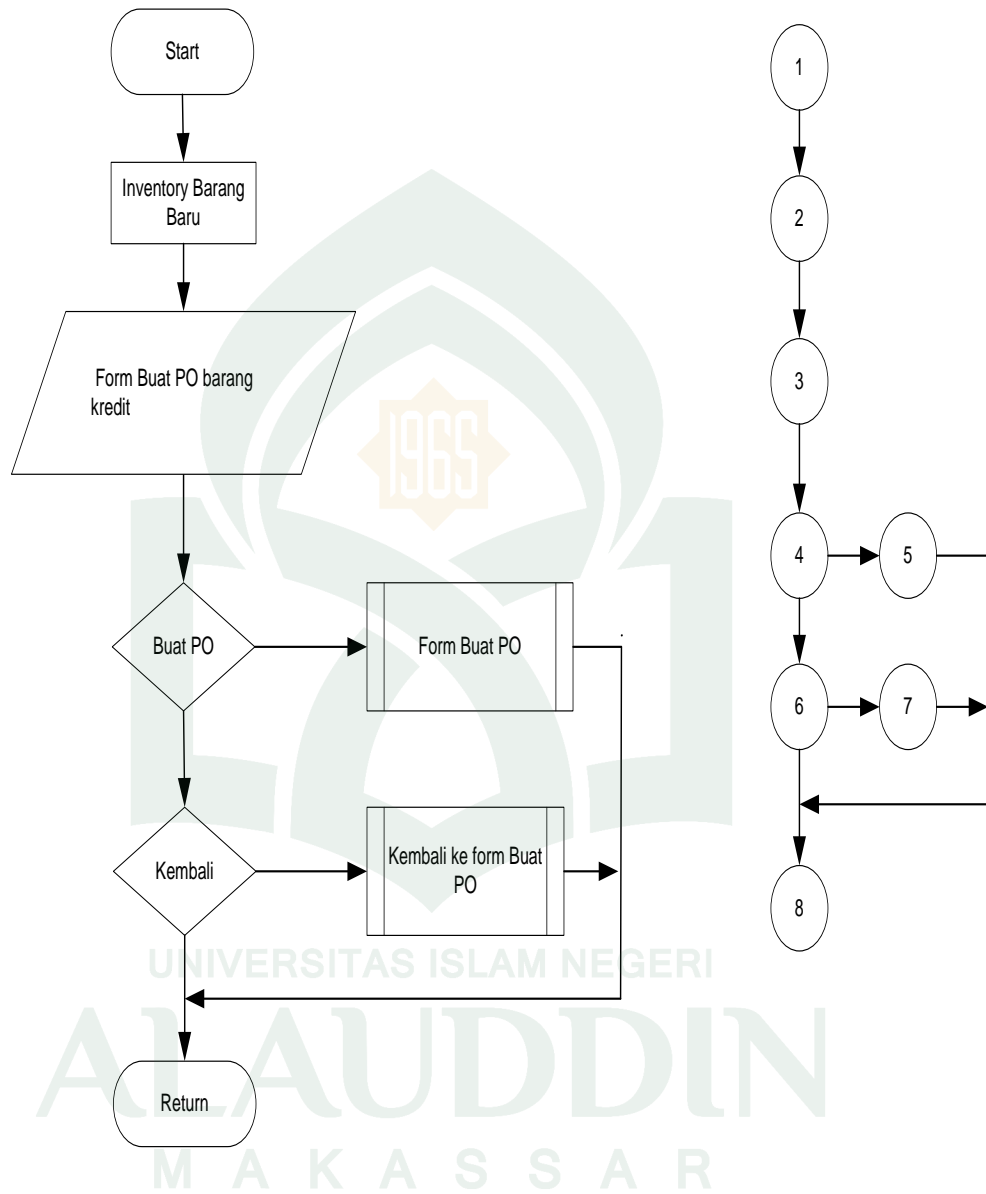
Gambar V.14 Flowchart dan Flowgraph Sub Menu Inventory Barang
