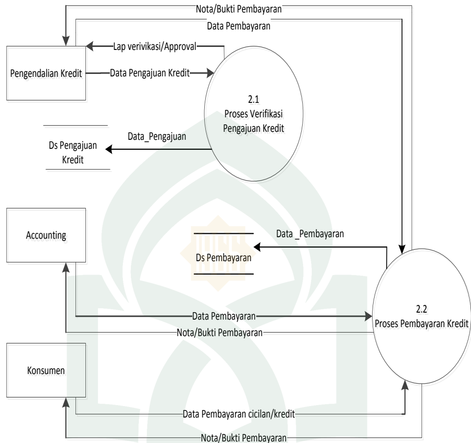
Gambar IV.7 Data Flow Diagram Level II Proses 2
