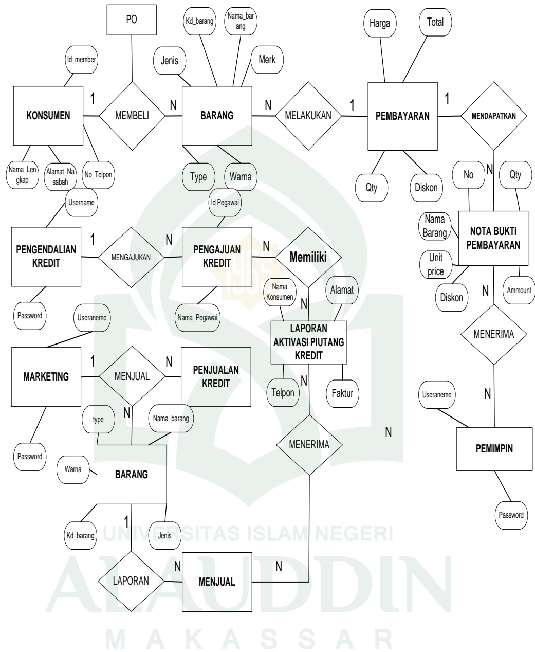
Gambar IV.9 Entity Relationship Diagram
