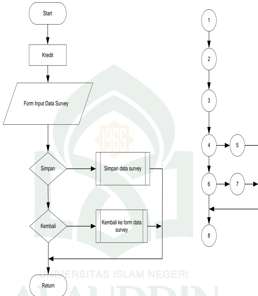
Gambar V.8 Flowchart dan Flowgraph Sub Menu Kredit Form Input Data Survey
