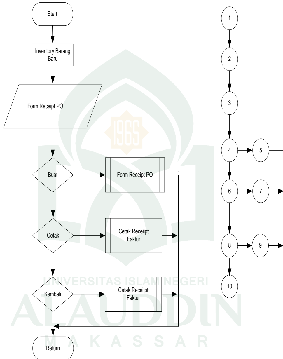
Gambar V.15 Flowchart dan Flowgraph Sub Menu Inventory Barang Baru Form Receipt PO
