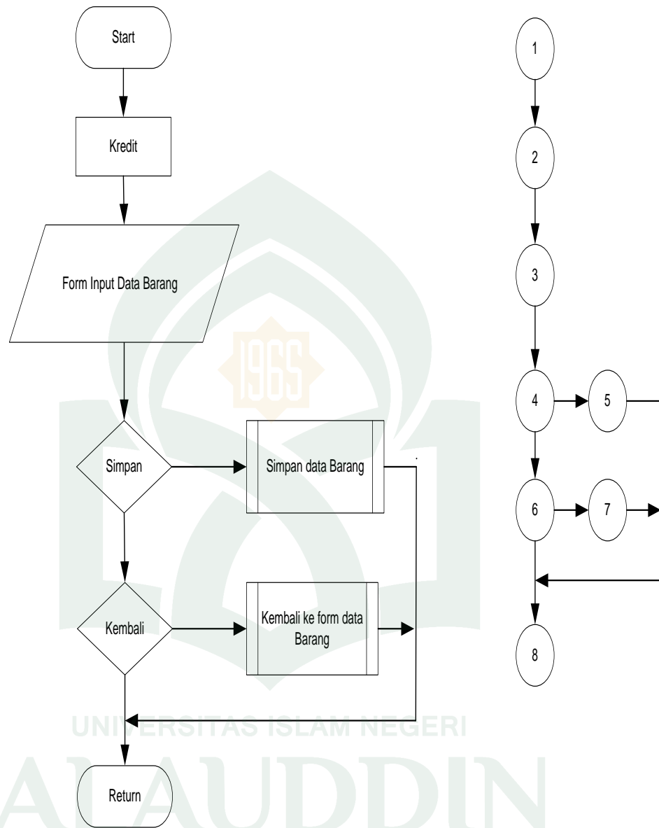
Gambar V.9 Flowchart dan Flowgraph Sub Menu Kredit Form Input
