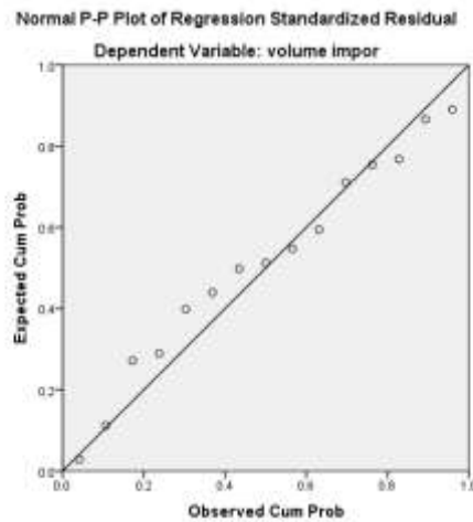
Gambar 4 Grafik Normal P - Plot
