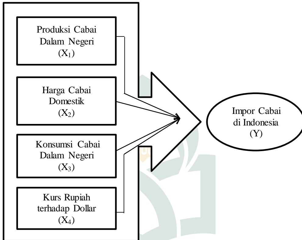
Gambar 2 MODEL PENELITIAN
