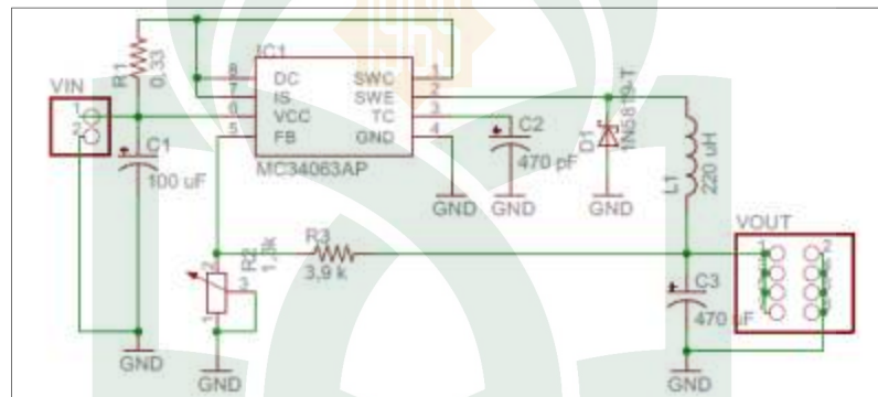
Gambar IV.3 Rangkaian Switching Regulator
