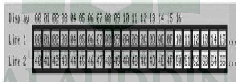
Gambar II.4 Data Register LCD
