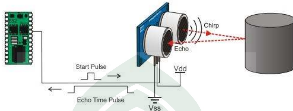
Gambar II.6 Sensor Ping
