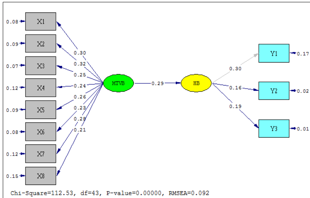
Gambar 4.8: Diagram Lintasan Basic Model-Estimates
