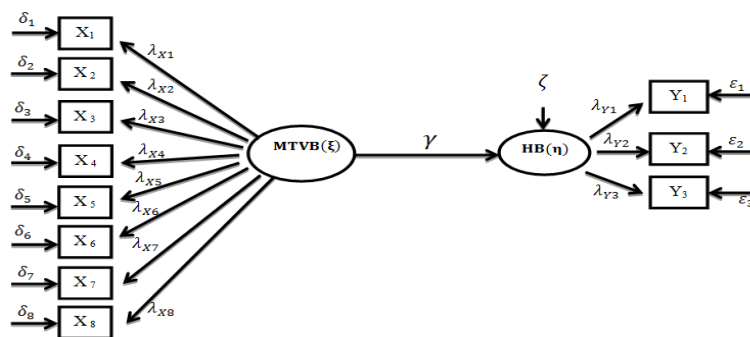
Gambar 3.1: Diagram Lintasan Model MTVB HB
