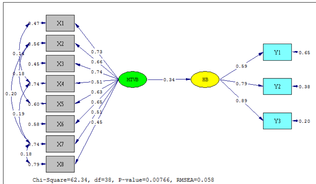
Gambar 4.10 : Diagram Lintasan Basic Model- Standardized Solution
