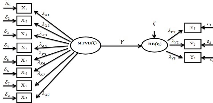
Gambar 3.3: full model MTVB HB
