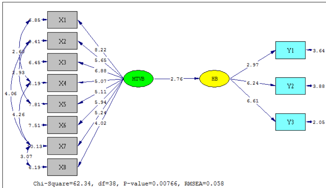
Gambar 4.9: Diagram lintasan basic model- t value
