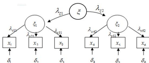
Fig. 2. Second-Order CFA
