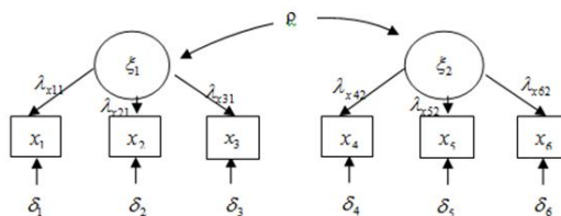
Fig. 1. First-Order CFA
