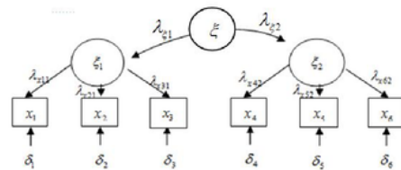
Fig. 2. Second-Order CFA
