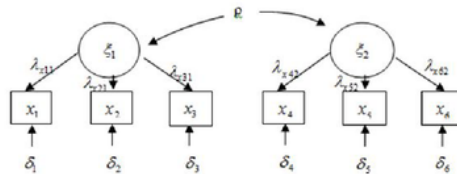
Fig. 1. First-Order CFA
