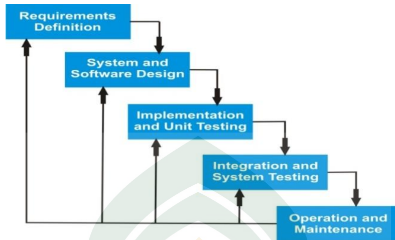
Gambar. 1 Model Waterfall I (Pressman, 2001).
