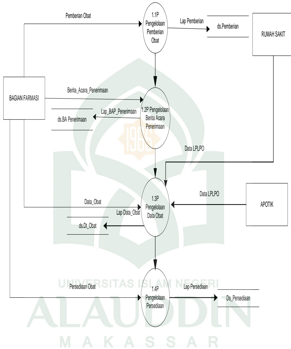
Gambar IV.6.Data Flow Diagram Level 1 Proses 1
