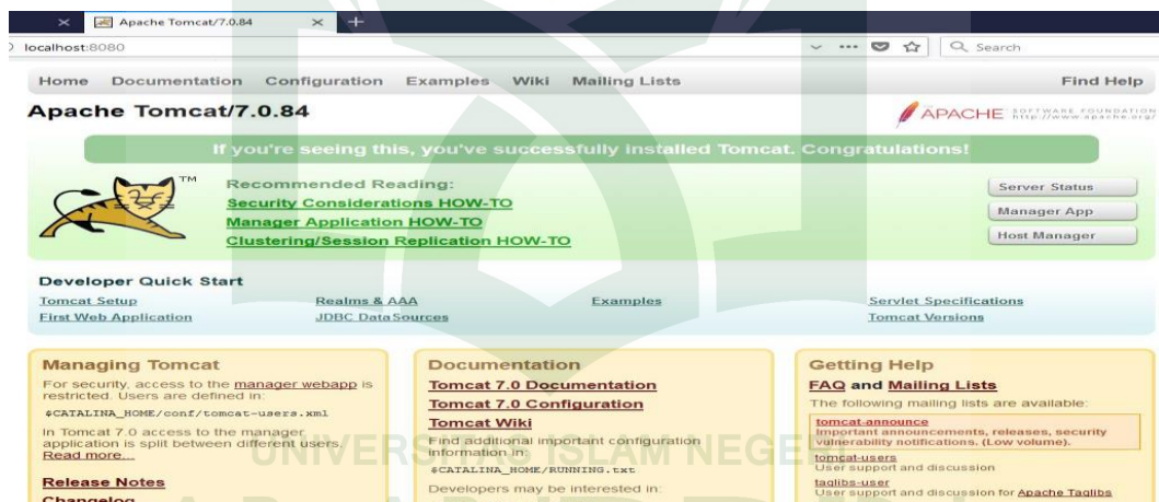
Gambar V.3 connect tomcat .
