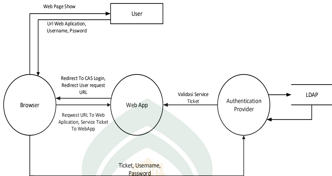
Gambar IV.5 DFD Level 1
