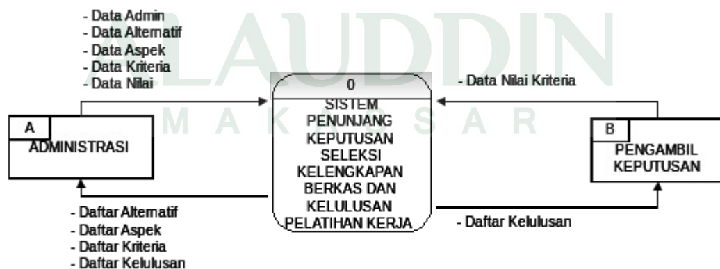
Gambar IV.6 Diagram Arus Data
