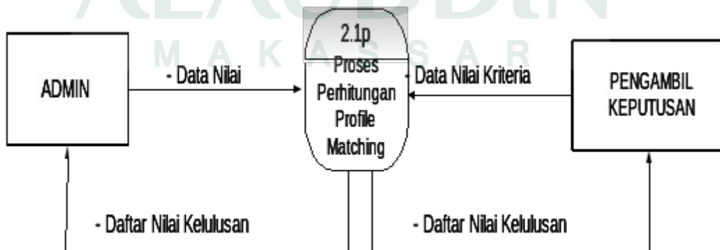
Gambar IV.9 Diagram Level 1 Proses 2
