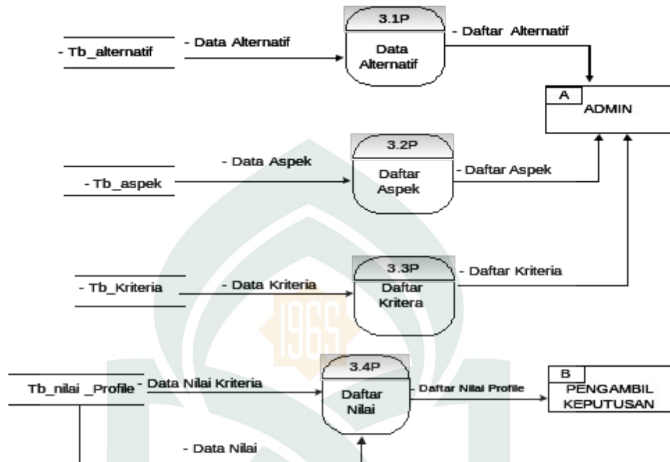
Gambar IV.10 Diagram Level 1 Proses 3
