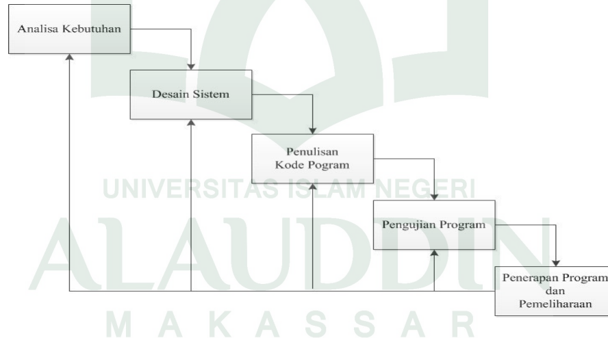
Gambar III.1 Metode Perancangan sistem Waterfall
