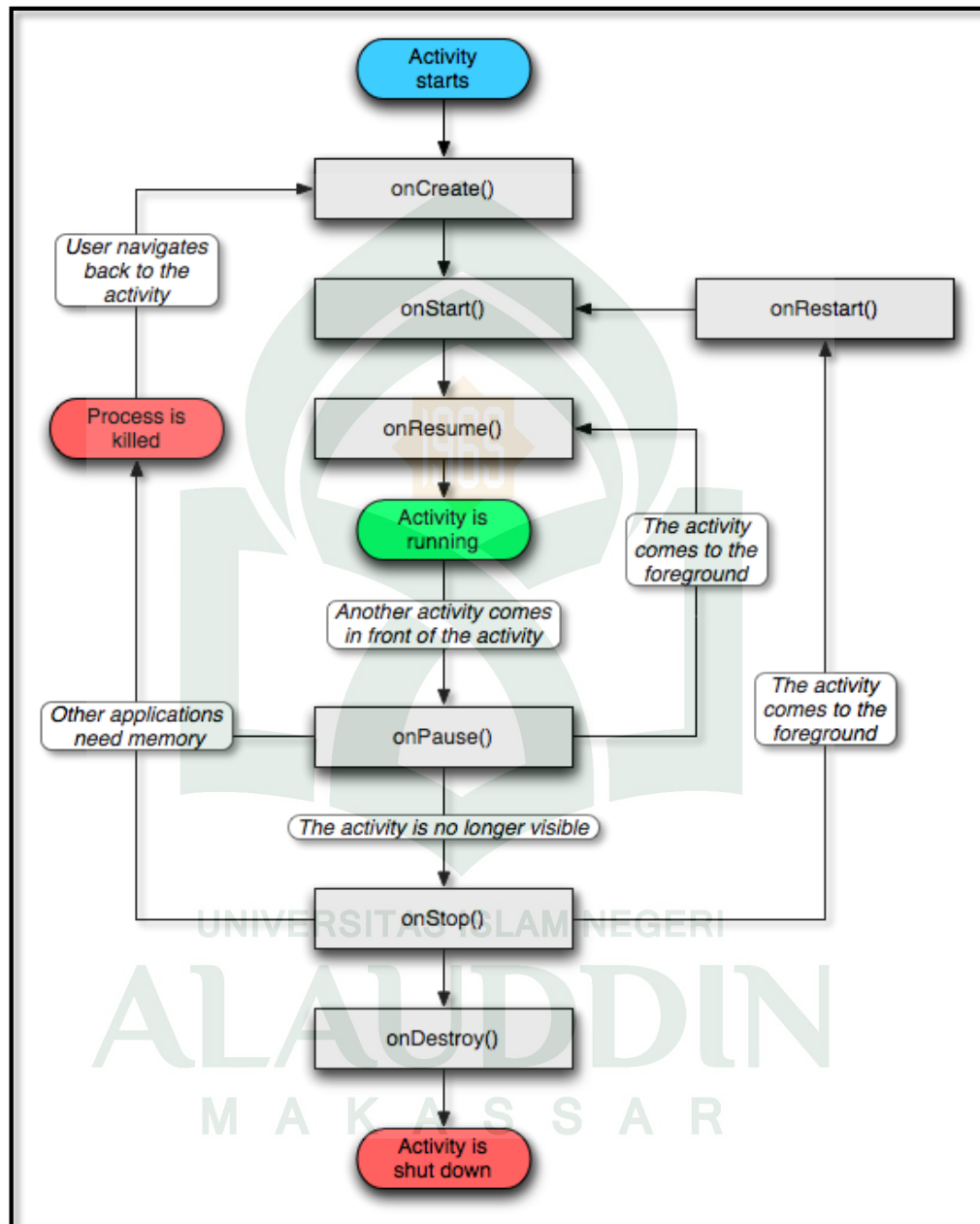
Gambar II.1 Siklus Hidup Activity (Wahana Komputer, 2013)
