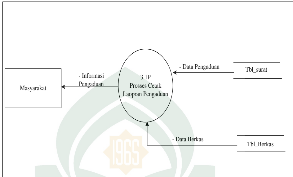
Gambar IV.7 Diagram Level 1 Proses 3
