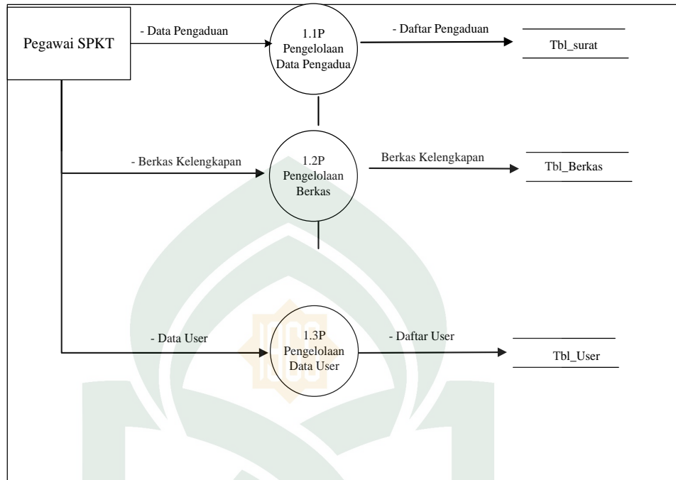
Gambar IV.5 Diagram Level 1 Proses 1
