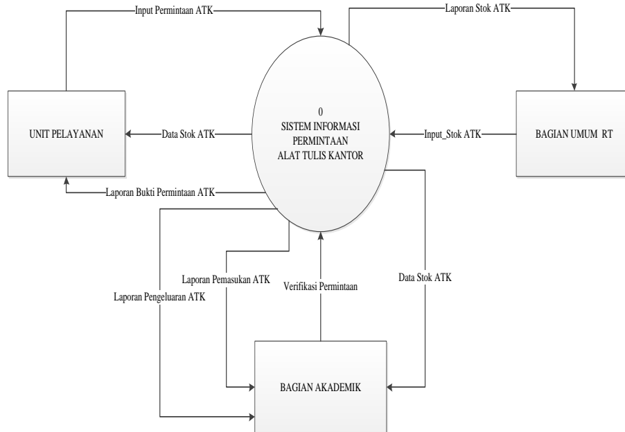
Gambar IV. 5. Diagram Level 0
