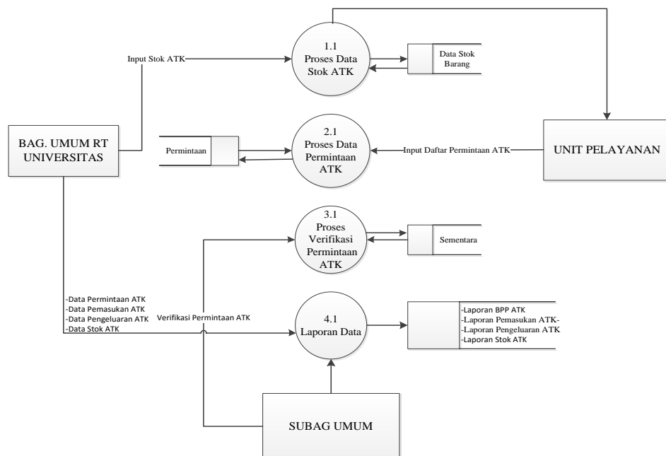
Gambar IV. 6. Diagram Level 1
