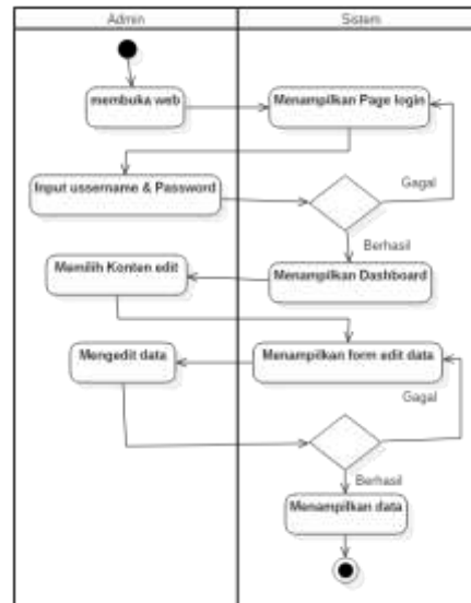
Gambar IV.17 Activity Diagram Edit Data Admin
