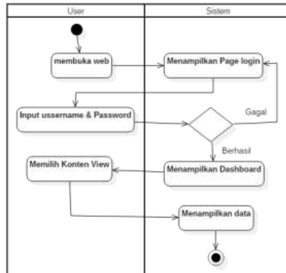
Gambar IV.15 Activity Diagram View Data User
