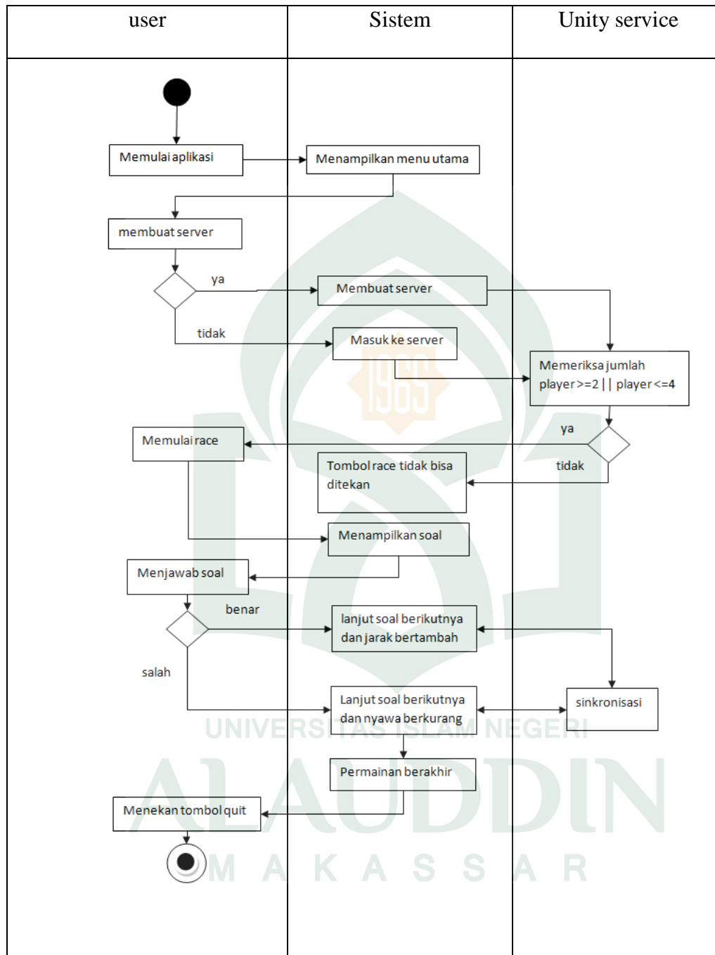
Gambar IV.5 Activity Diagram Menu Gameplay
