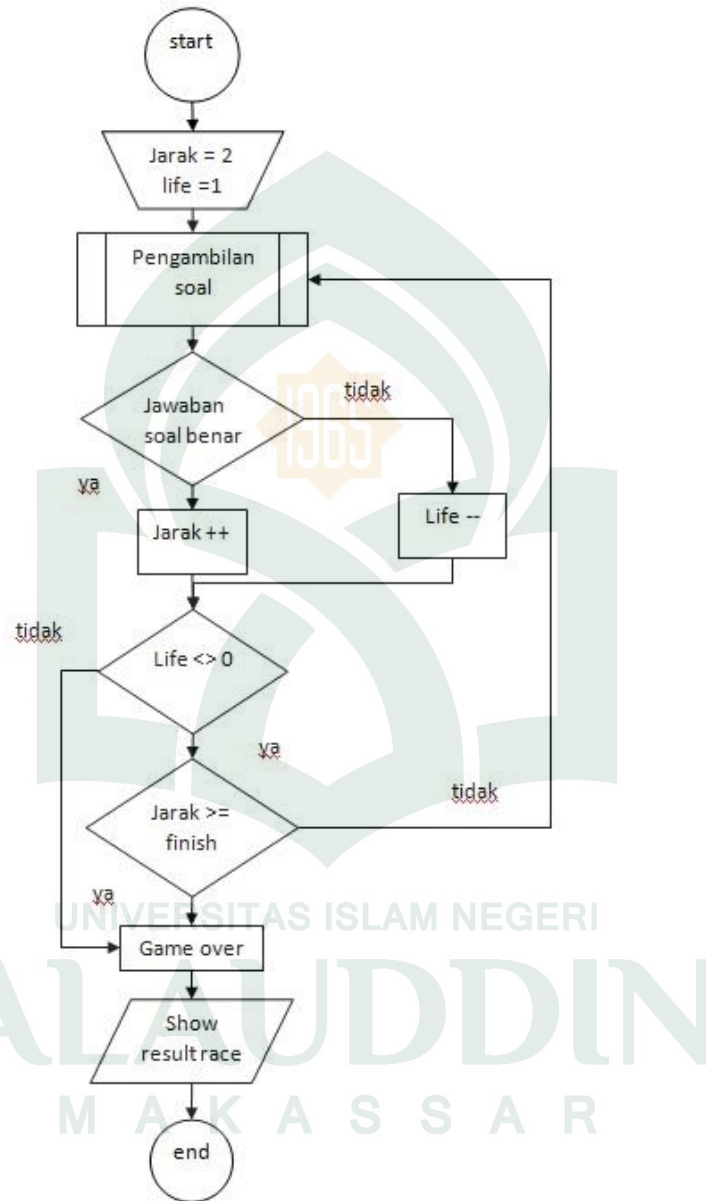
Gambar IV.6 Flowchart prosedur gameplay
