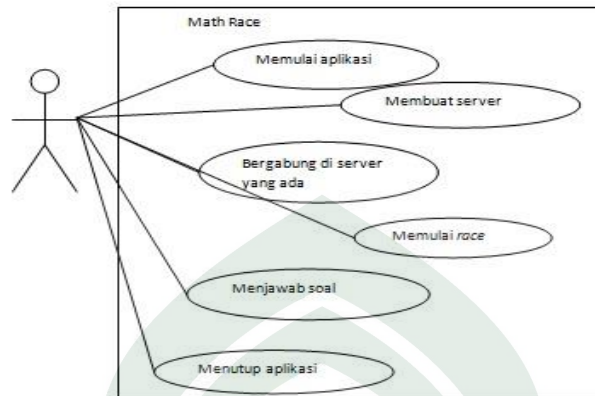
Gambar IV.3 Use Case Diagram
