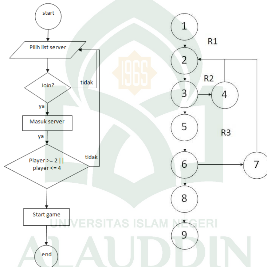
Gambar V.3 Flowchart dan Flowgraph prosedur join server
