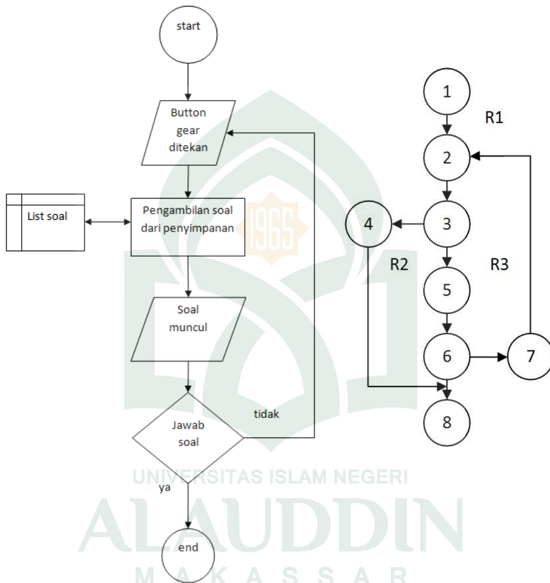
Gambar V.1 Flowchart dan Flowgraph prosedur pengambilan soal
