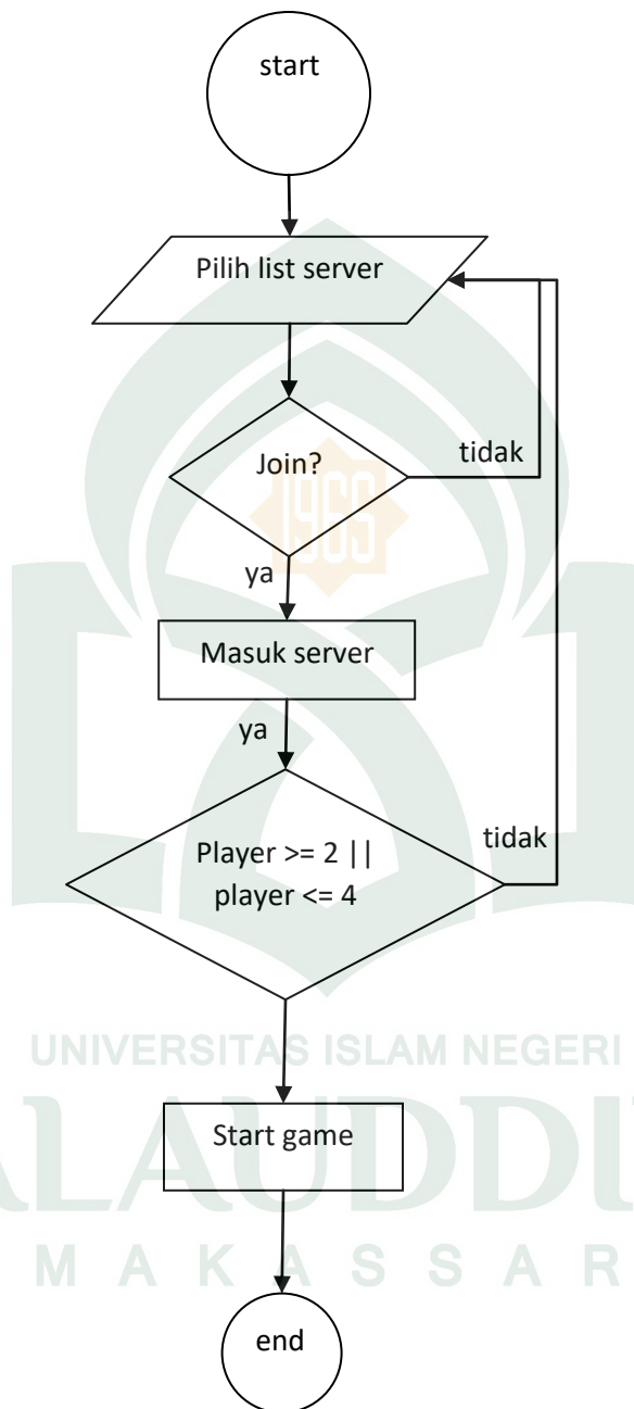
Gambar IV.7 Flowchart prosedur join server
