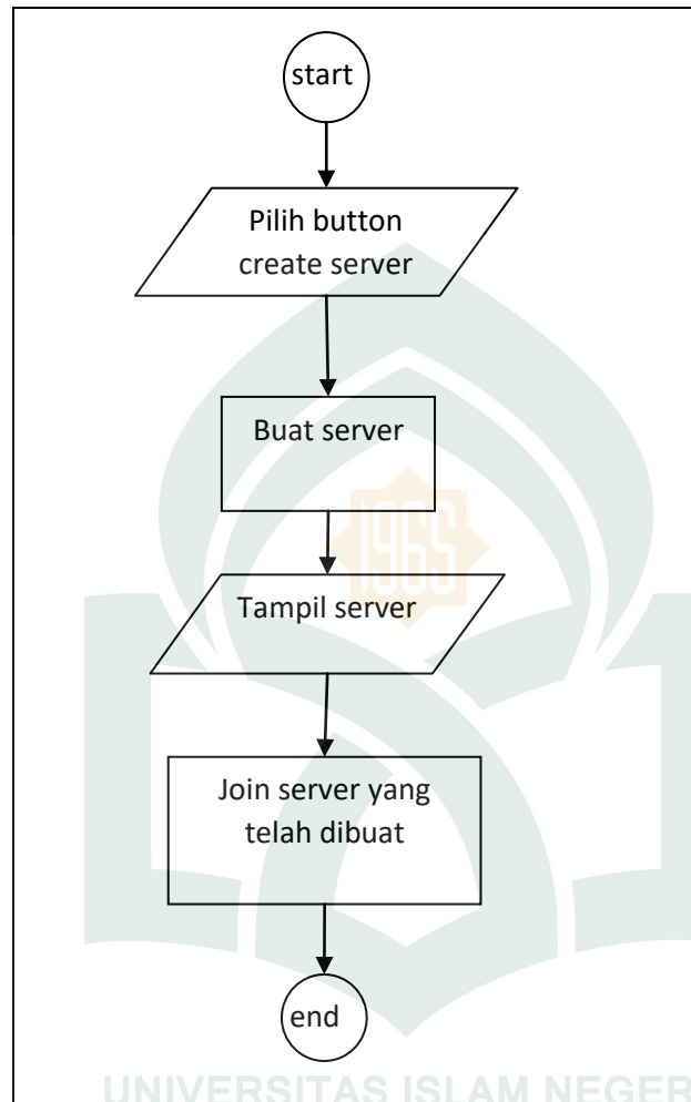
Gambar IV.9 Flowchart prosedur create server
