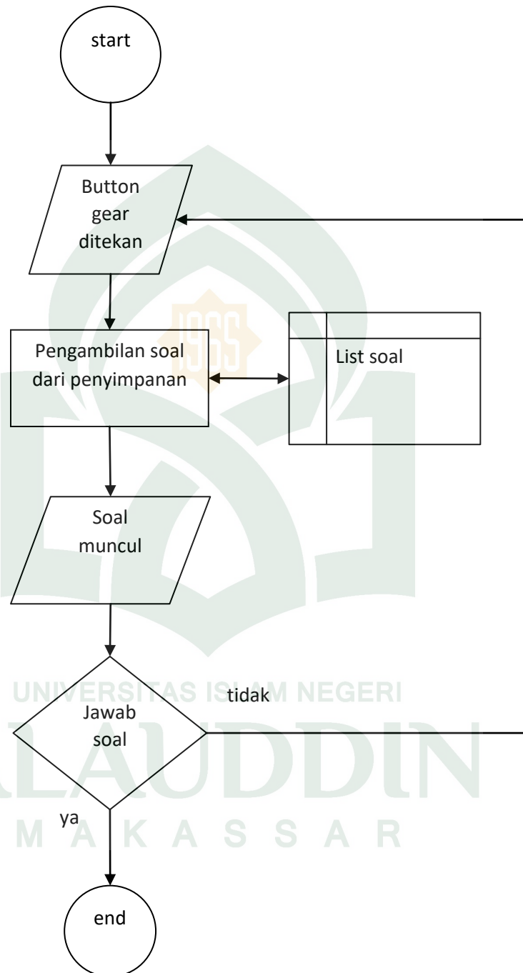
Gambar IV.8 Flowchart prosedur pengambilan soal
