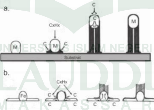
Gambar 2.10 Mekanisme Pertumbuhan CNT (a) Tip Growth , (b) Base Growth
