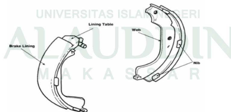
Gambar II.3: Brake Shoe dan Lining Rem Tromol (Siahaan dan Yung Sen, 2008)
