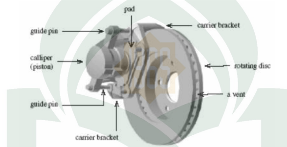
Gambar II.1: Rem Cakram (Siahaan dan Yung Sen, 2008)
