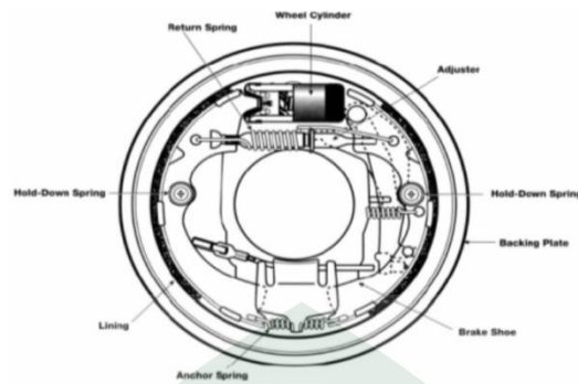
Gambar II.2: Rem Tromol (Siahaan dan Yung Sen, 2008)
