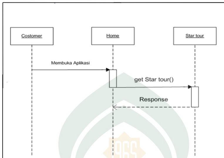
Gambar IV.5 Sequence Diagram menu Home
