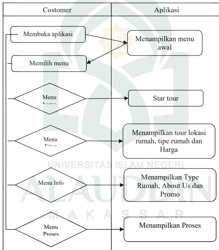
Gambar IV. 9 Activity Diagram
