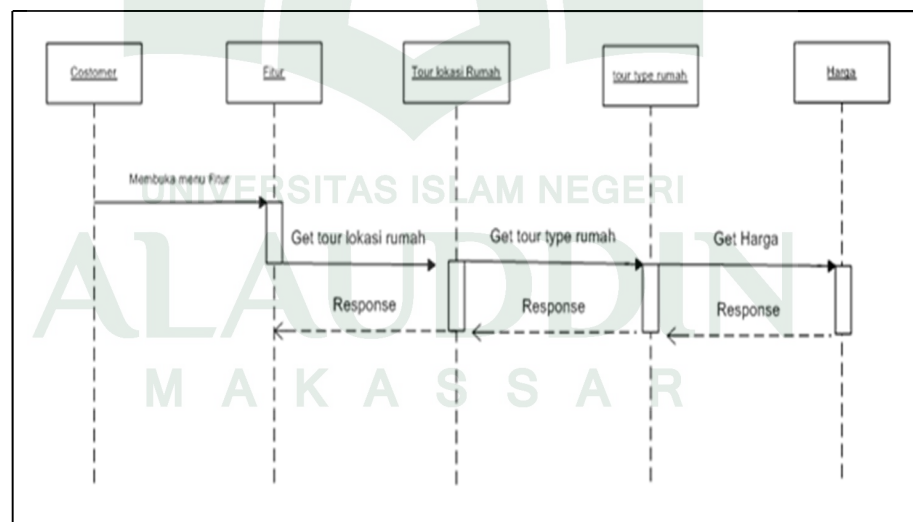
Gambar IV.6 Sequence Diagram menu Fitur
