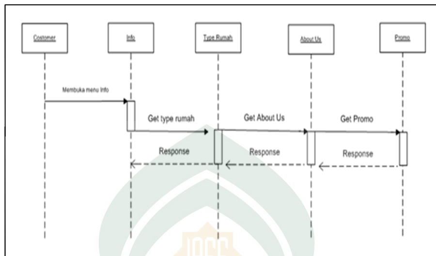
Gambar IV.7 Sequence Diagram menu info
