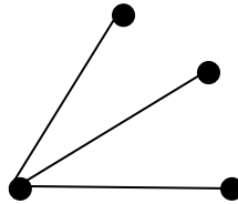
Gambar 4.5 Subgraf H_4 .
