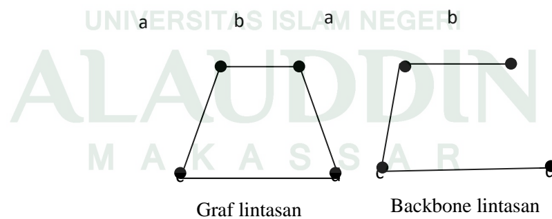
Gambar 2.21. Backbone Lintasan
