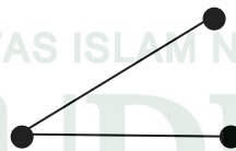
Gambar 4.4 Subgraf H_3 .
