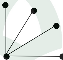
Gambar 4.6 Subgraf H_5 .
