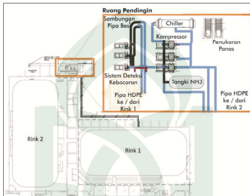
Gambar 53. Skema pendinginan lantai ice skating
