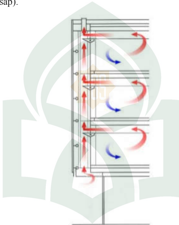
Gambar 20. Extract air system
