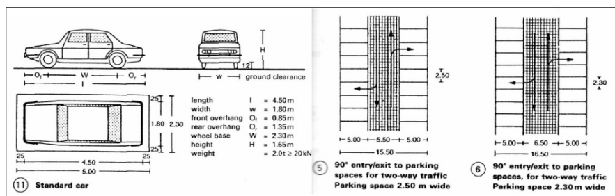
Gambar 52. Standar parkir Sumber : Neufert architect's Data
