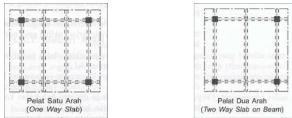
Gambar 68. Sistem lantai (Juwana, 2010)
