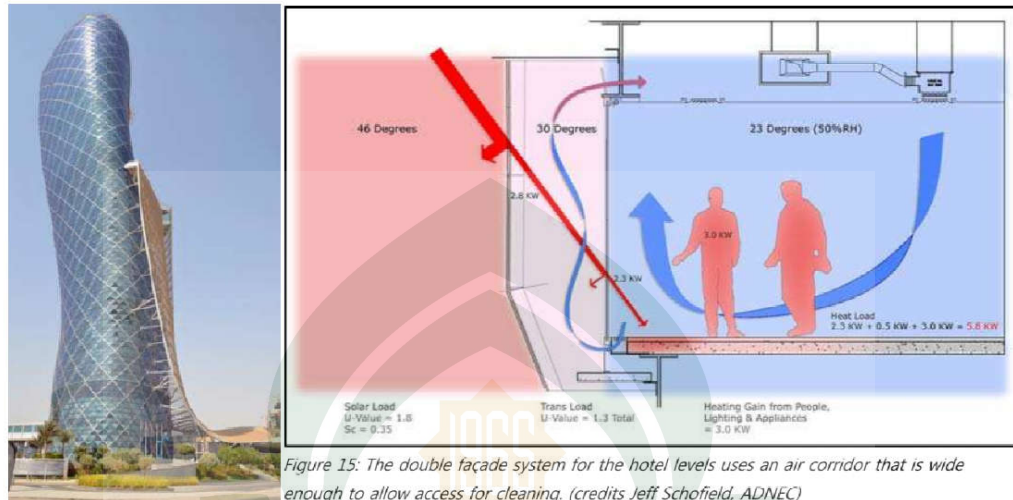
Gambar 22. Double Facade System
