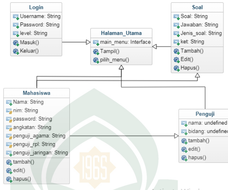
Gambar IV.4 Class Diagram
