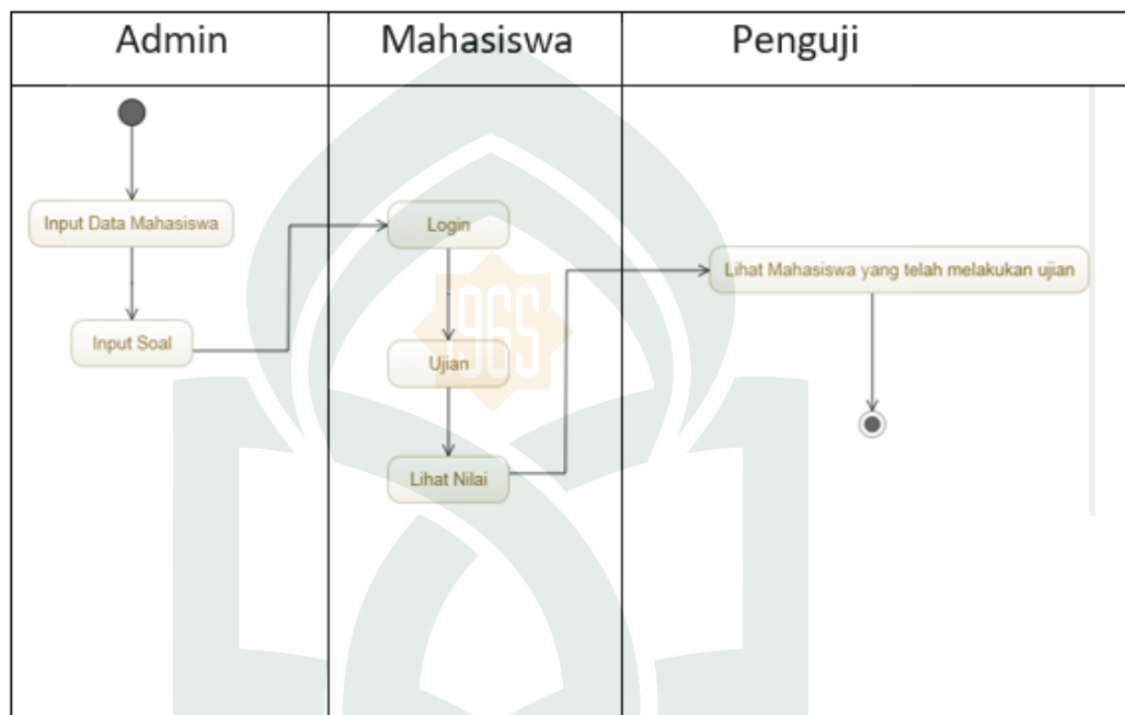
Gambar IV.9 Activity Diagram
