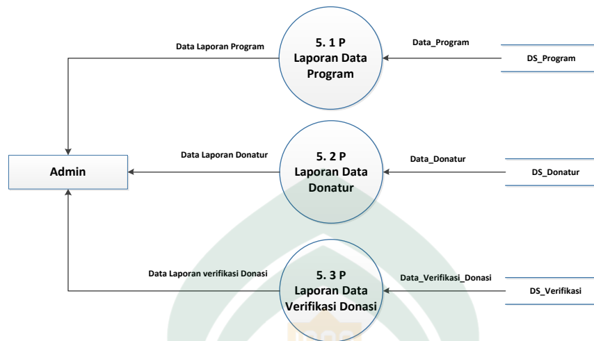
Gambar IV.6. Data Flow Diagram Level 5 Proses 2
