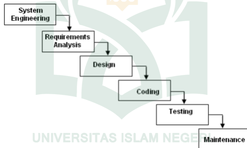
Gambar III. 1. Model Waterfall
