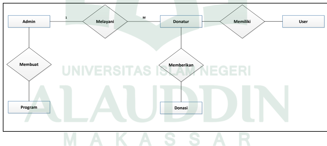
Gambar IV.7. Entity Relationship Diagram (ERD)
