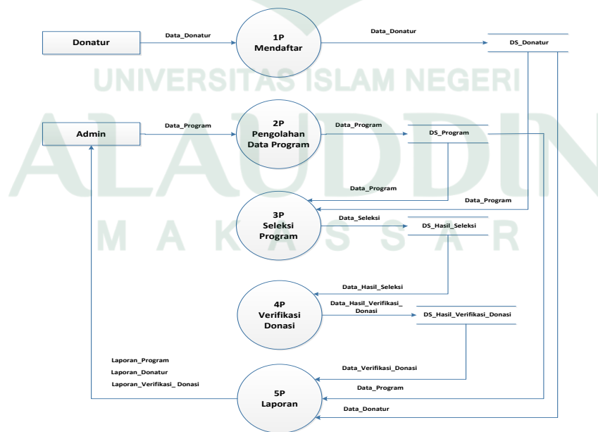
Gambar IV.5. Data Flow Diagram Level 1
