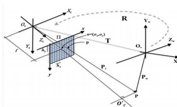
Gambar II.1 Pin-hole Model (Cyganek, 2009)
