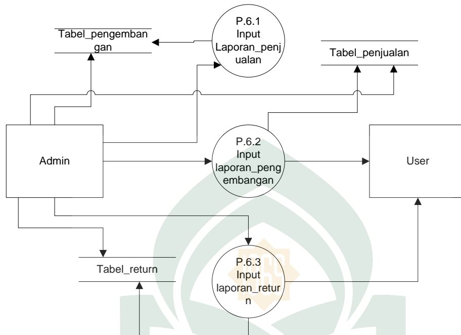
Gambar IV.9. Data flow Diagram level 2 proses 4
