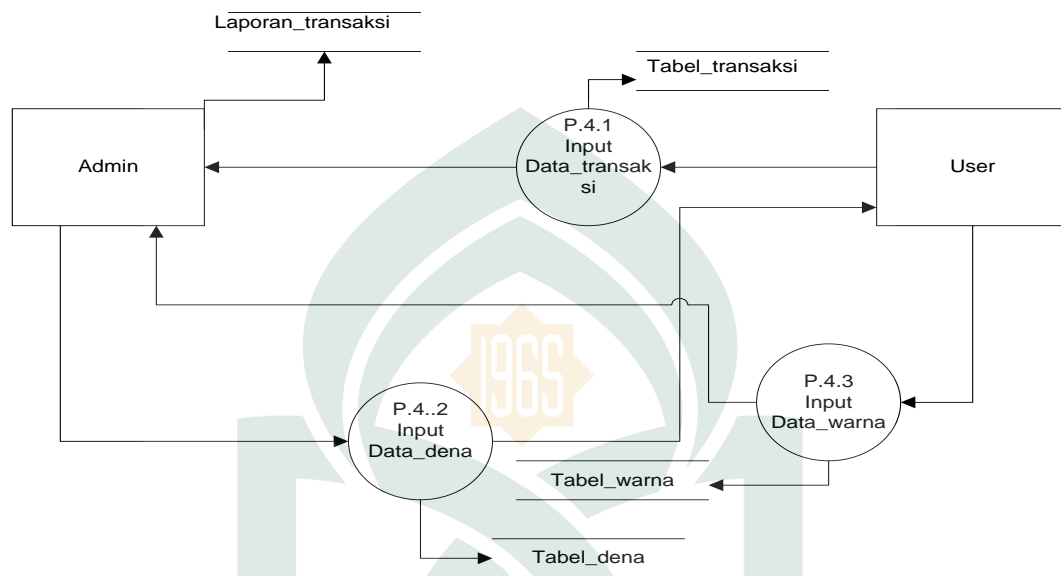
Gambar IV.7. Data flow Diagram level 2 proses 4
