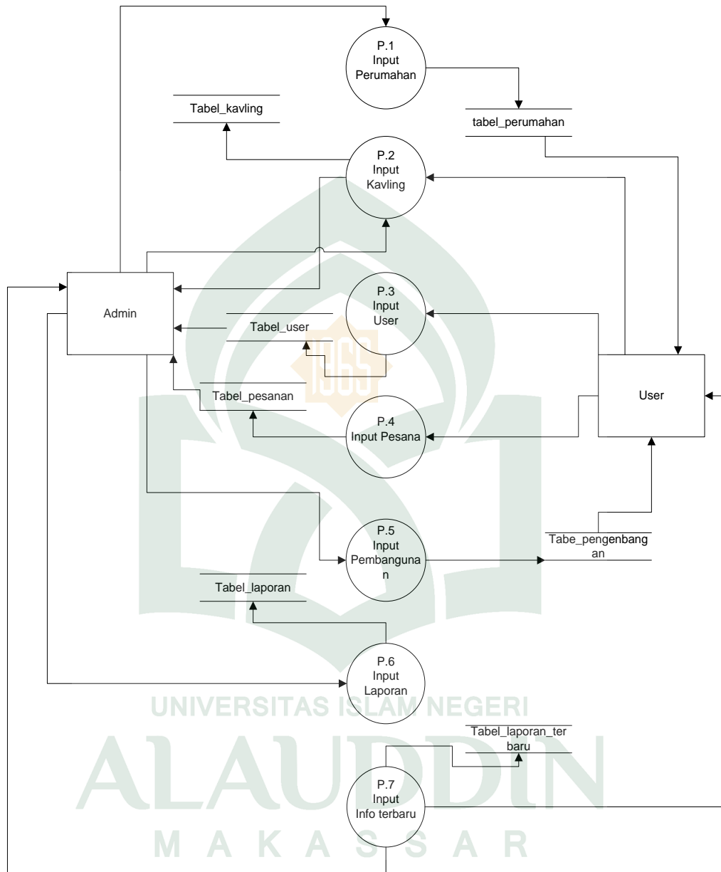
Gambar IV.6. Data Flow Diagram Level
