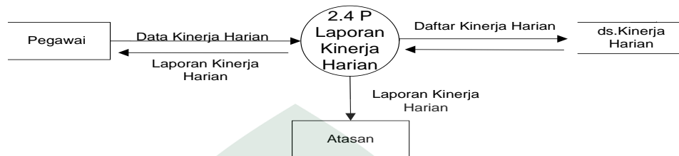
Gambar IV.6 Diagram Level 2 Peroses 4
