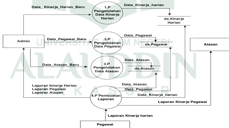
Gambar IV.4 Diagram Level 1
