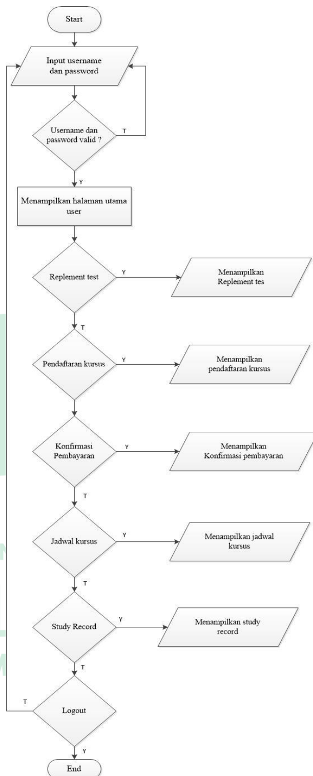
Gambar IV.13 Flowchart
