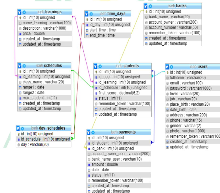
Gambar IV.5 Class Diagram
