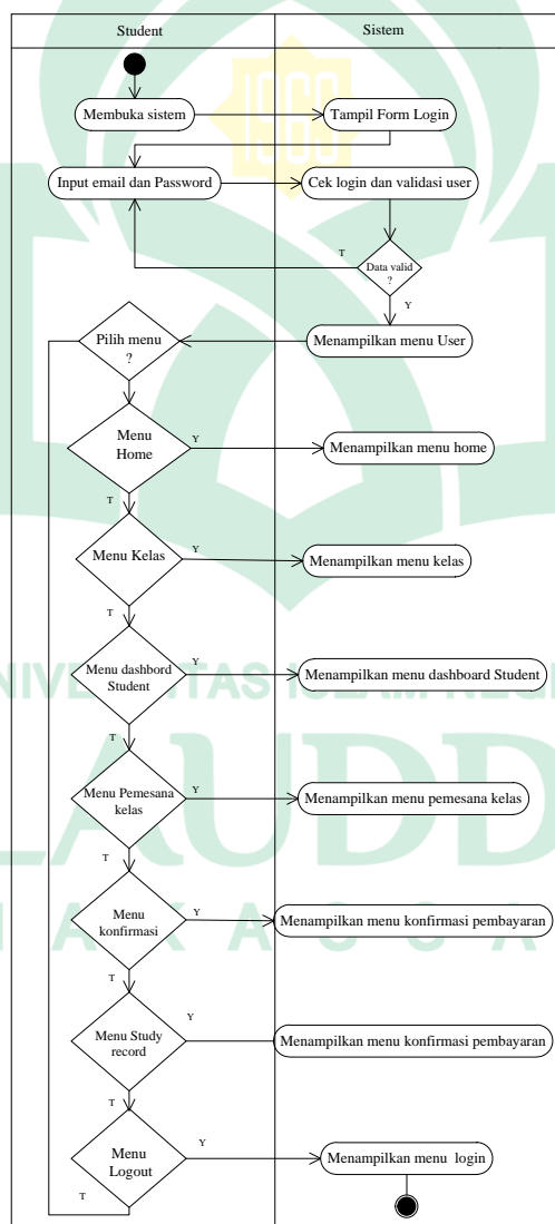
Gambar IV.11 Activity Diagram
