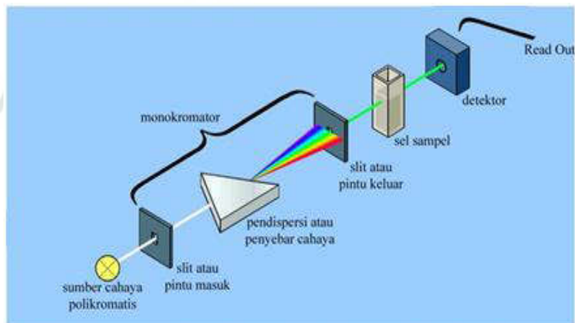
Gambar 2.13. Cara Kerja Alat UV-Vis ( Ultraviolet Visible )
