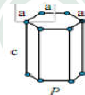
Gambar 2.12. Sistem hexagonal
