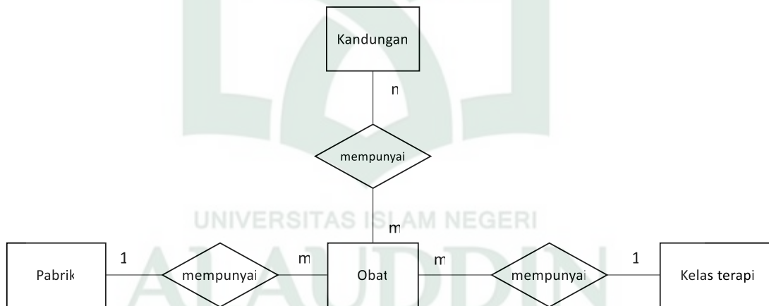
Gambar IV.11 Entity Relationship Diagram
