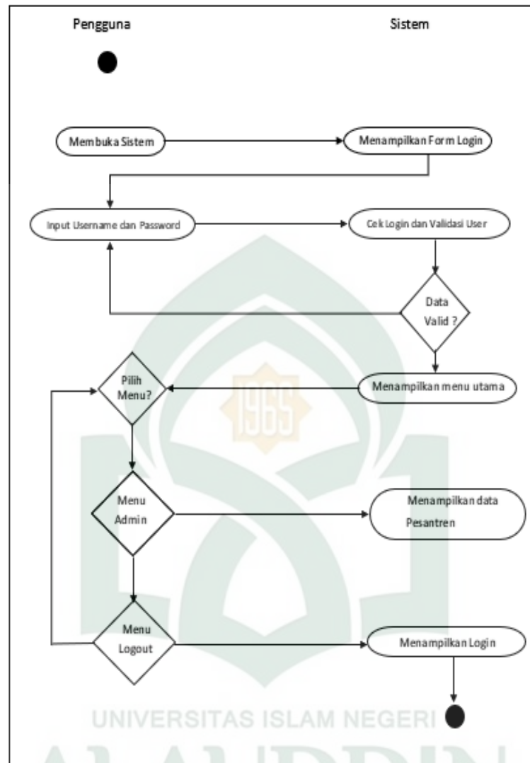
Gambar IV.9 Activity Diagram
