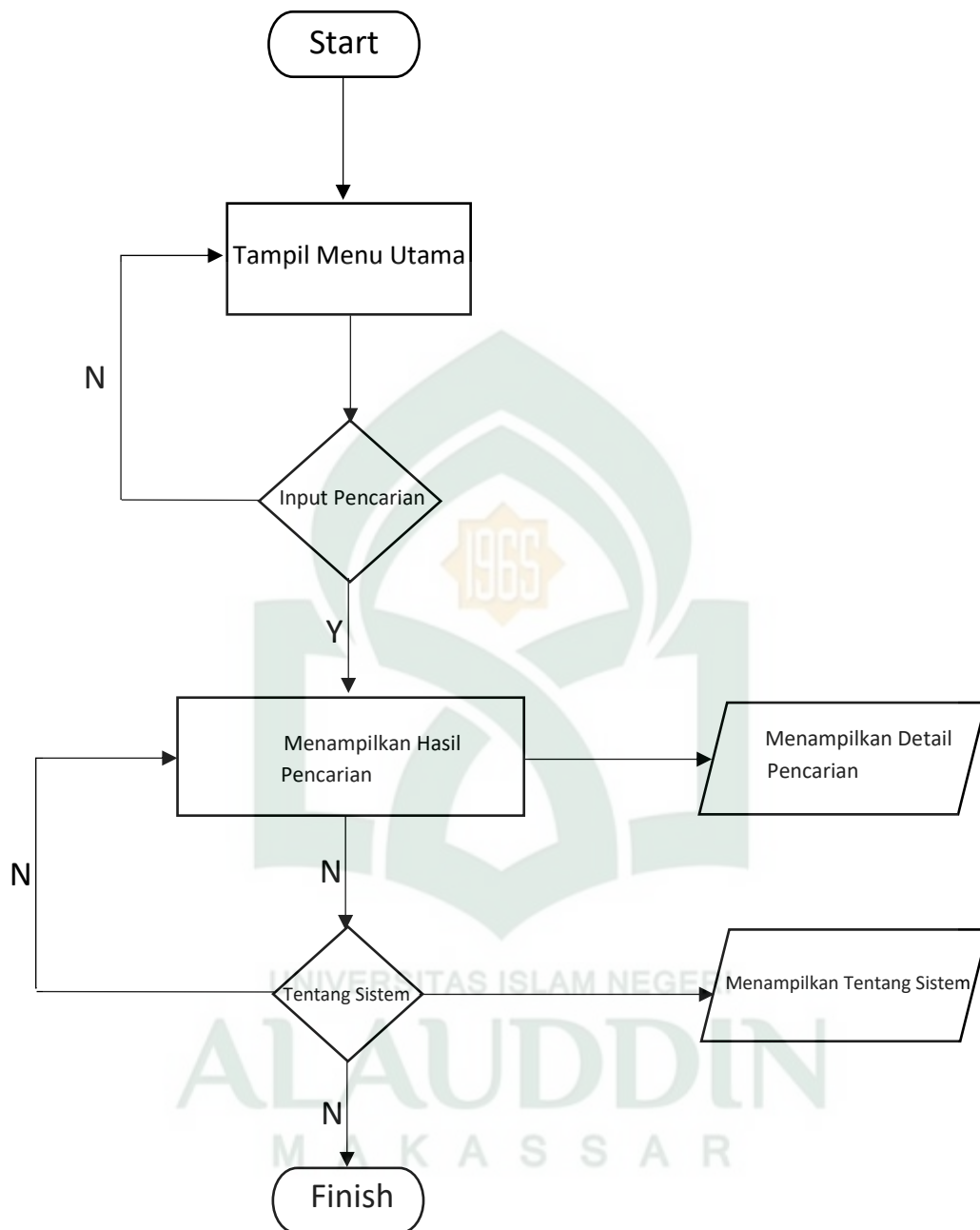
Gambar IV.10 Flowchart
