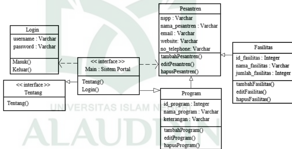
Gambar IV.5 Class Diagram
