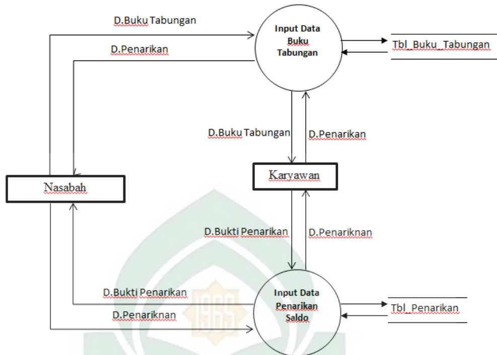
Gambar IV.8 Data Flow Diagram (DFD) Level 2 Layanan Penarikan Saldo
