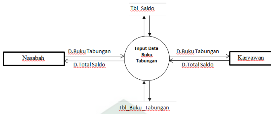
Gambar IV.10 Data Flow Diagram (DFD) Level 2 Layanan Cek Saldo
