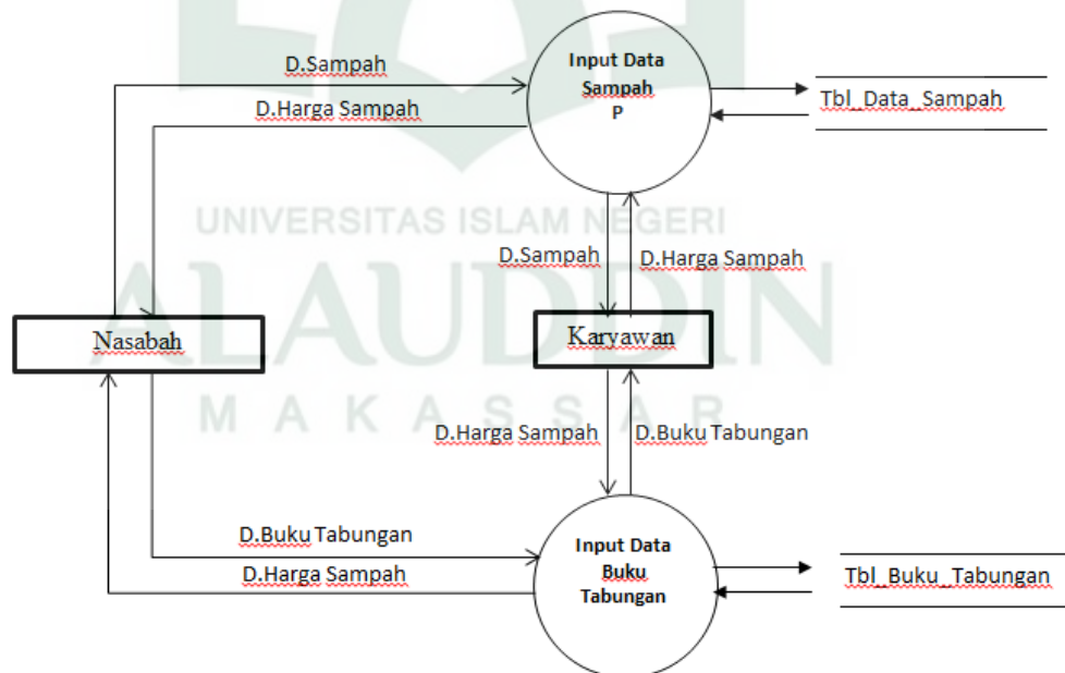
Gambar IV.7 Data Flow Diagram (DFD) Level 2 Layanan Penimbangan
