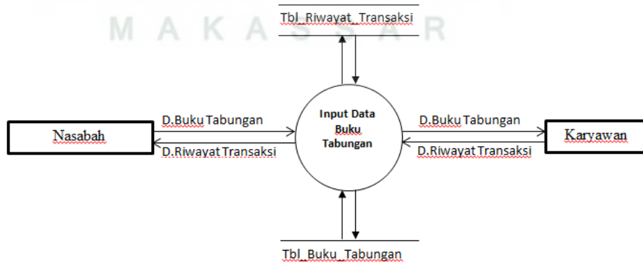
Gambar IV.12 Data Flow Diagram (DFD) Level 2 Layanan Mutasi Rekening
