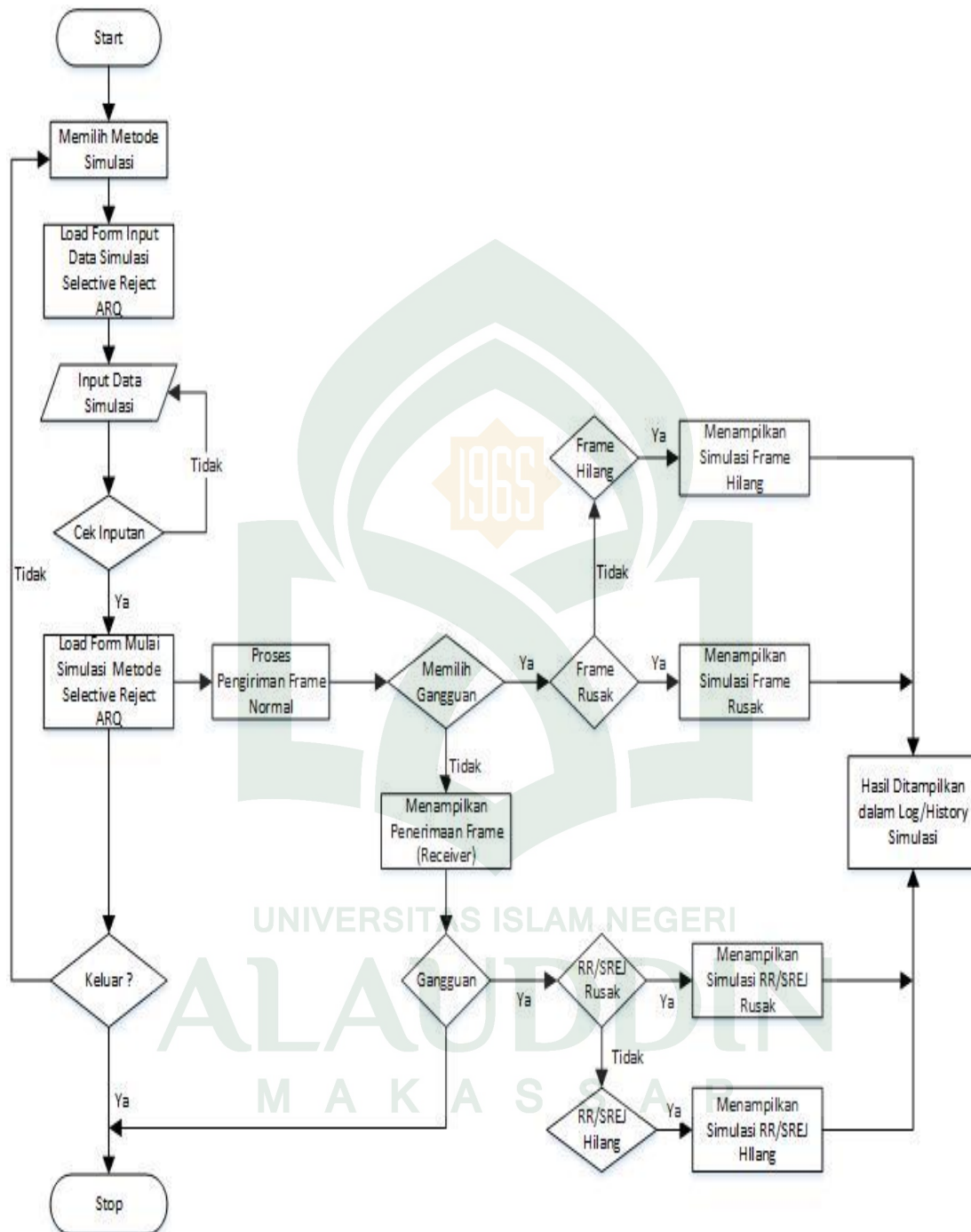
Gambar IV.17 Flowchart Simulasi Metode Selective Reject ARQ
