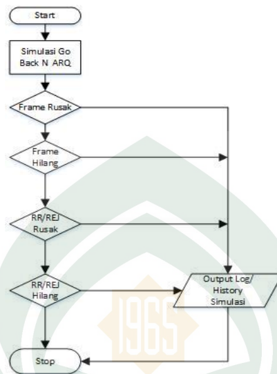
Gambar V.18 Flowchart Simulasi Go back N ARQ
