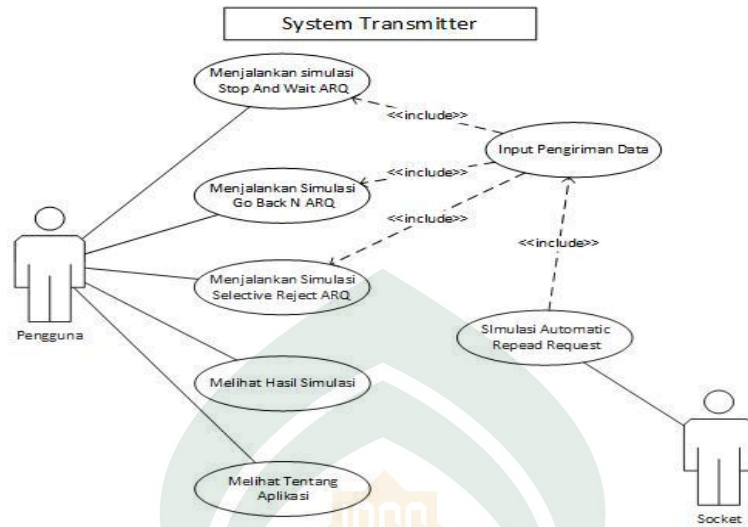
Gambar IV.3 Use Case Diagram Transmitter
