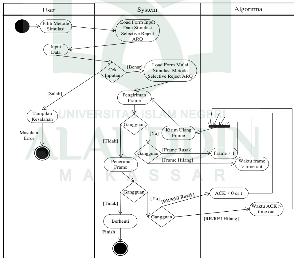
Gambar IV.14 Activity Diagram Simulasi Metode Selective Reject ARQ
