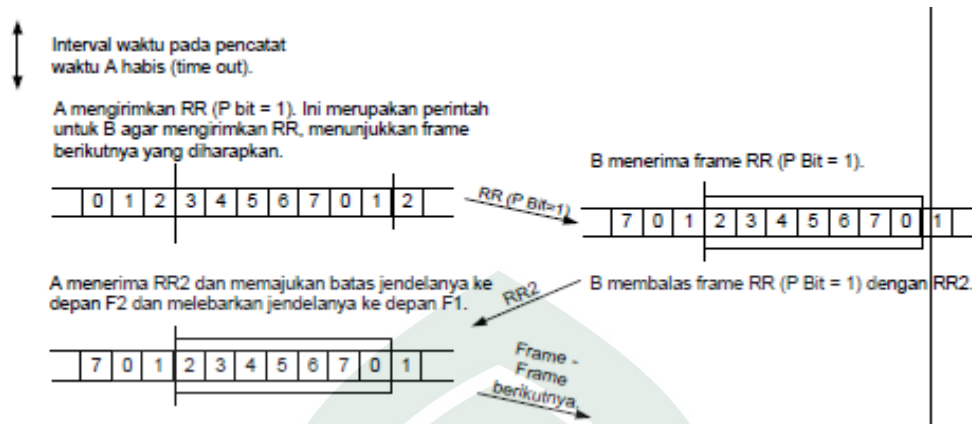
Gambar II.7 Gambaran kasus Metode Selective-Reject ARQ (Stallings, 2001a)
