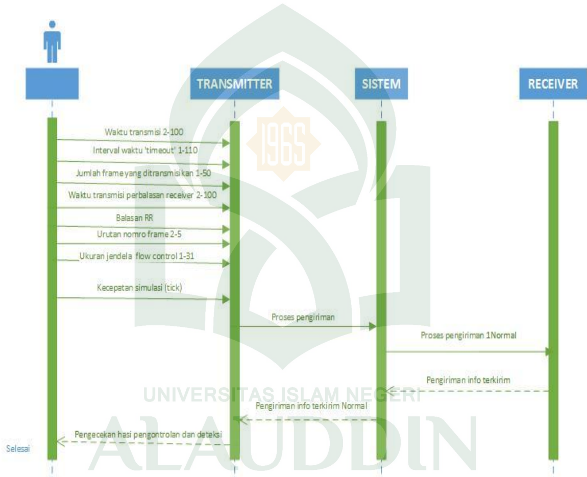
Gambar IV.8 Sequence Diagram Metode Go-Back-N ARQ Normal
