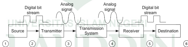
Gambar II. 2 Rincian Proses Pengiriman Data (Stallings, 2001a)
