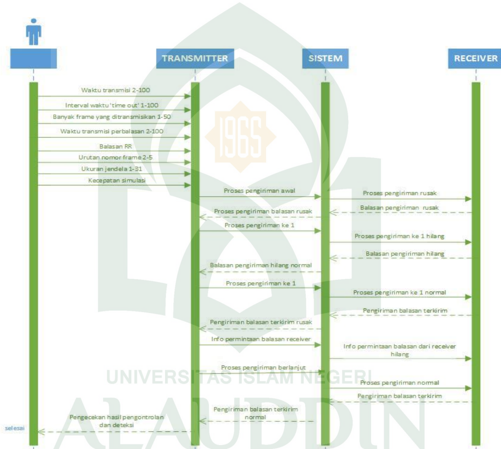
Gambar IV.11 Sequence Diagram Metode Selective-Reject ARQ Tidak Normal
