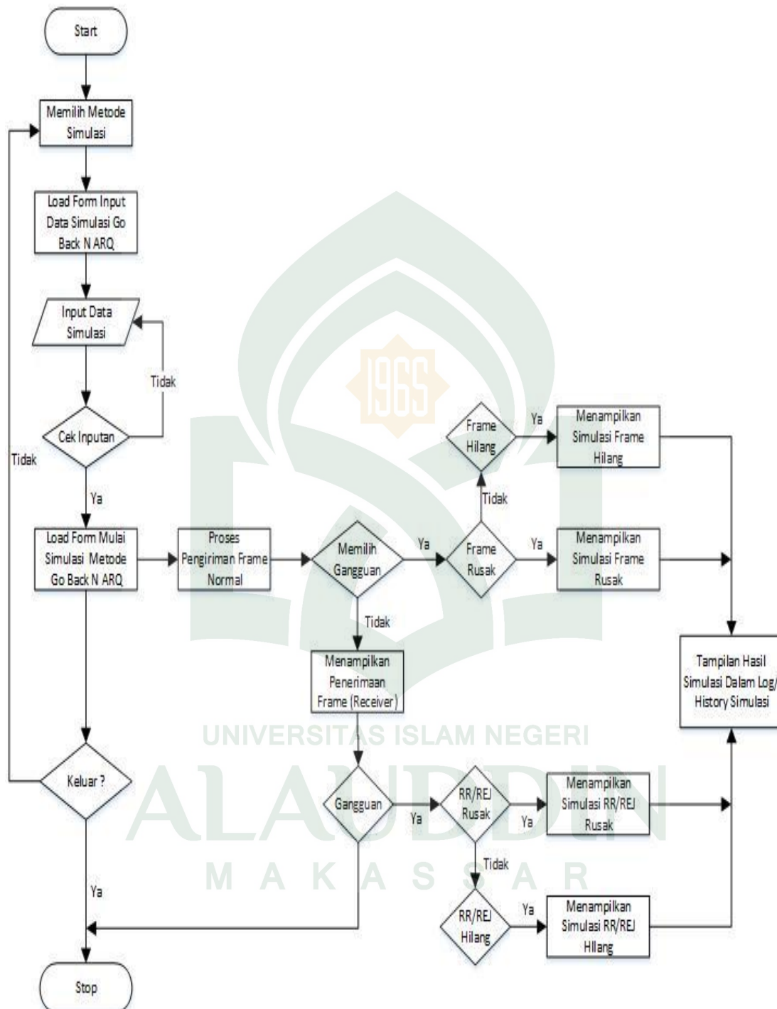
Gambar IV.16 Flowchart Simulasi Metode Go Back N ARQ
