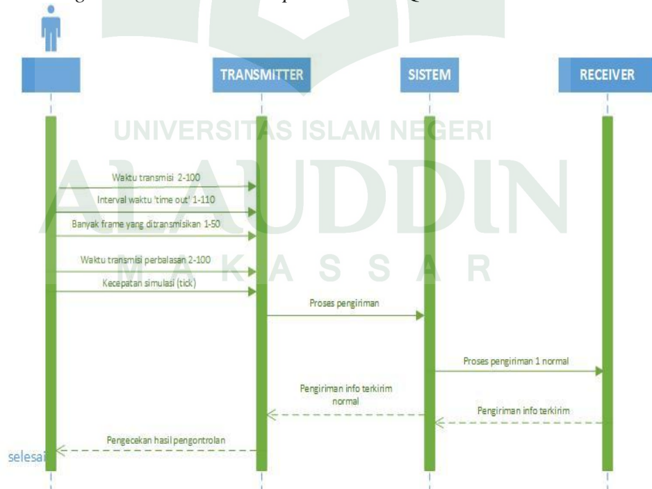
Gambar IV.6 Sequence Diagram metode Stop-N-Wait ARQ Normal
