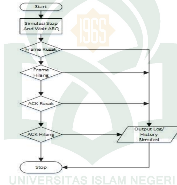
Gambar V.16 Flowchart Simulasi Stop And Wait ARQ
