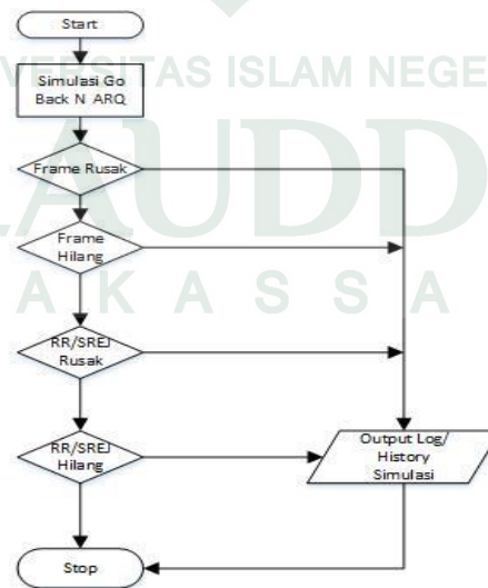
Gambar V.20 Flowchart Simulasi Selective Reject ARQ
