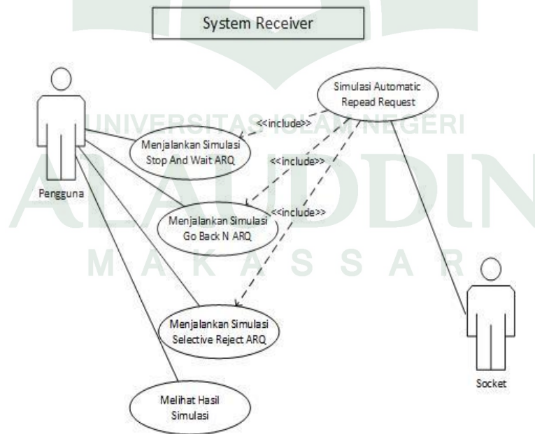
Gambar IV.4 Use Case Diagram Receiver
