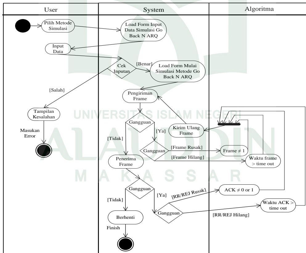
Gambar IV.13 Activity Diagram Simulasi Metode Go Back N ARQ
