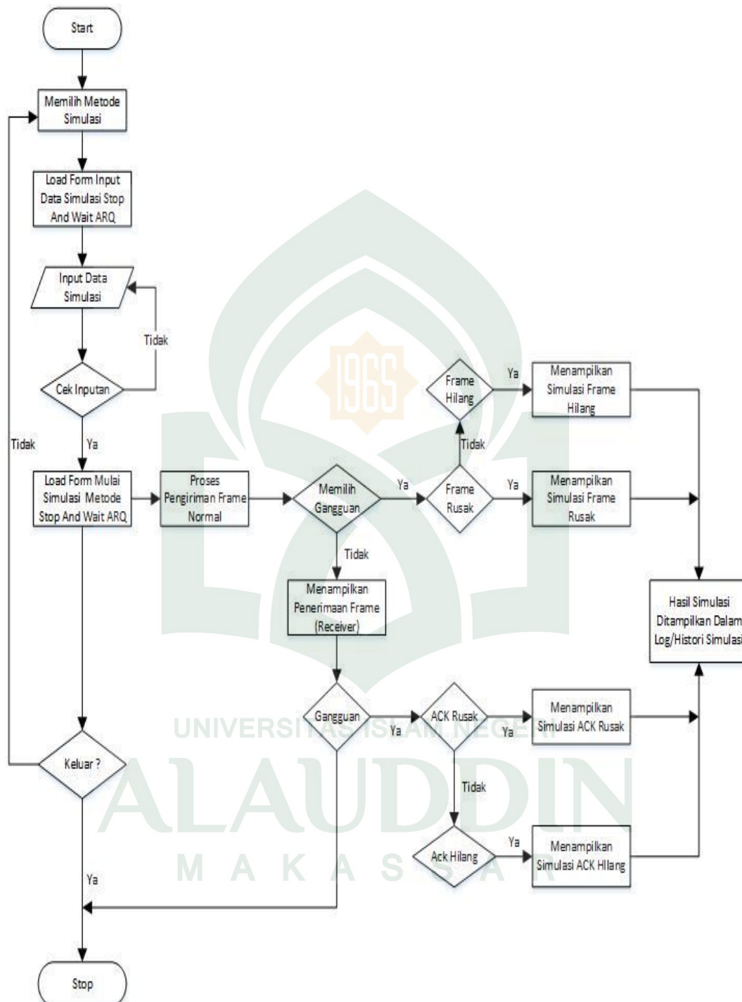
Gambar IV.15 Flowchart Simulasi Metode Stop And Wait ARQ
