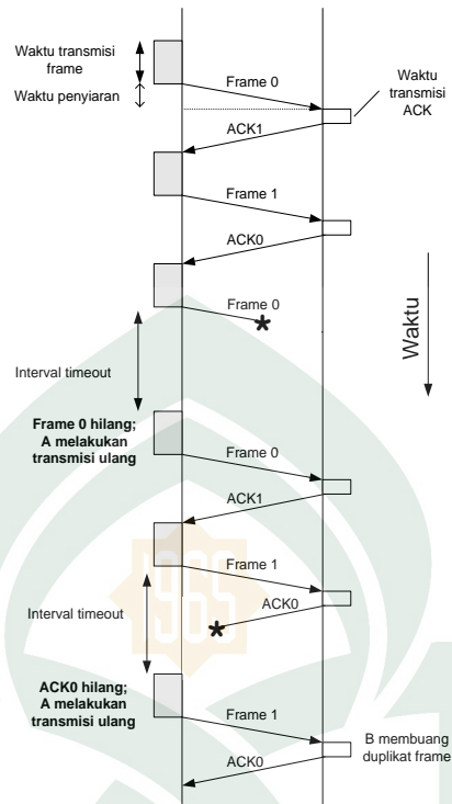
Gambar II. 5 Ilustrasi Prosedur Stop-and-Wait ARQ (Stallings, 2001a)
