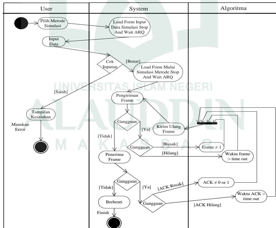
Gambar IV.12 Activity Diagram Simulasi Metode Stop and Wait ARQ
