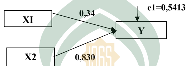
Gambar 4.3 Diagram Jalur Model I
