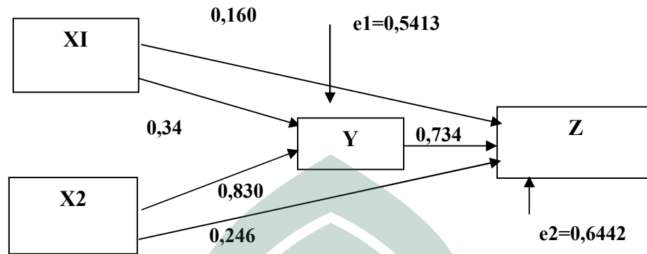
Gambar 4.4 Diagram Jalur Model II
