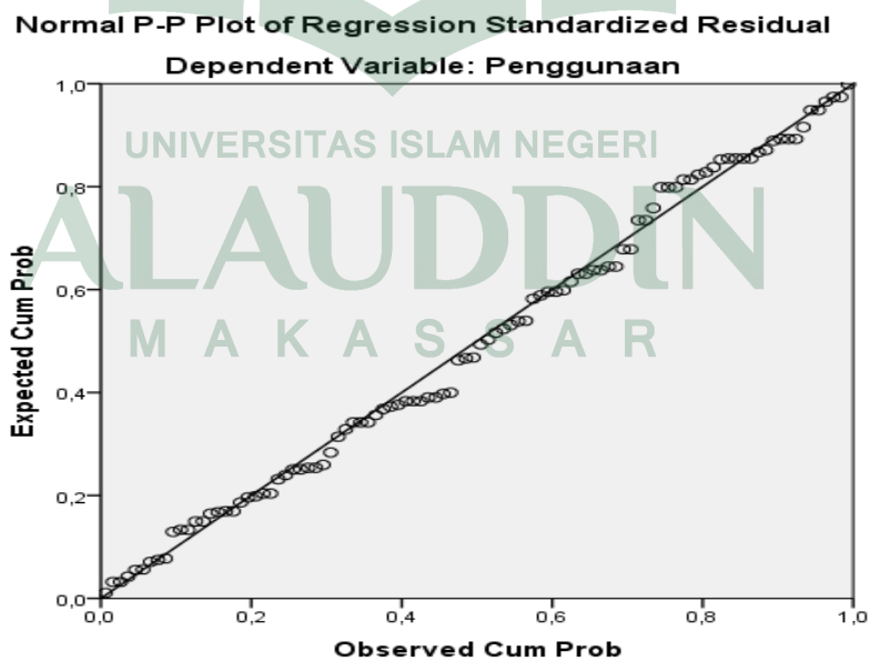
Gambar 4.2 Hasil Uji Normalitas Model II
