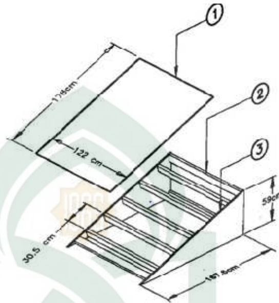
Gambar II. 20 Detail rangka Launch Ramp Sumber : Secrets of Skateboarding 2008, diakses 12 November 2014
