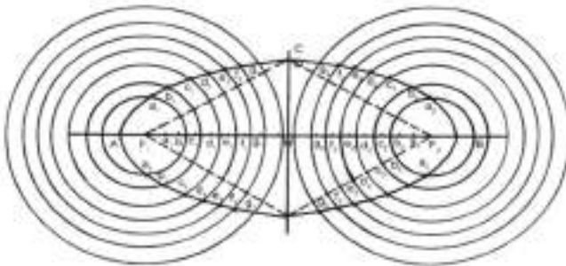
Gambar 30 Elips (Cara I)
