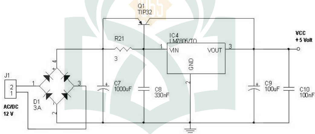
Gambar IV.4 Rangkaian Power Supply .
